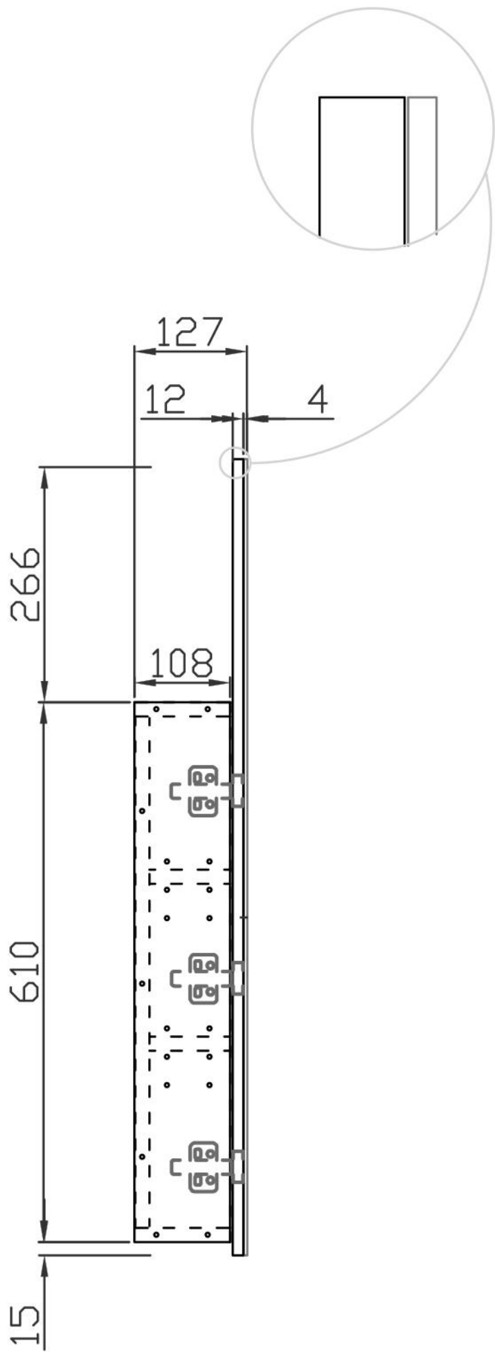
Front View
