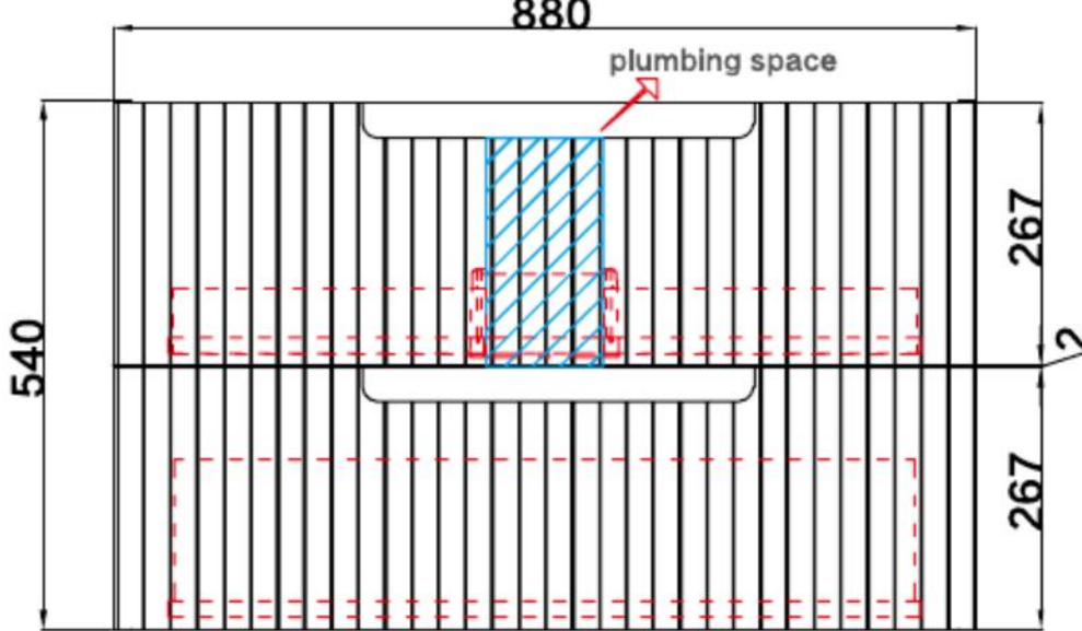
CAWH42-900
