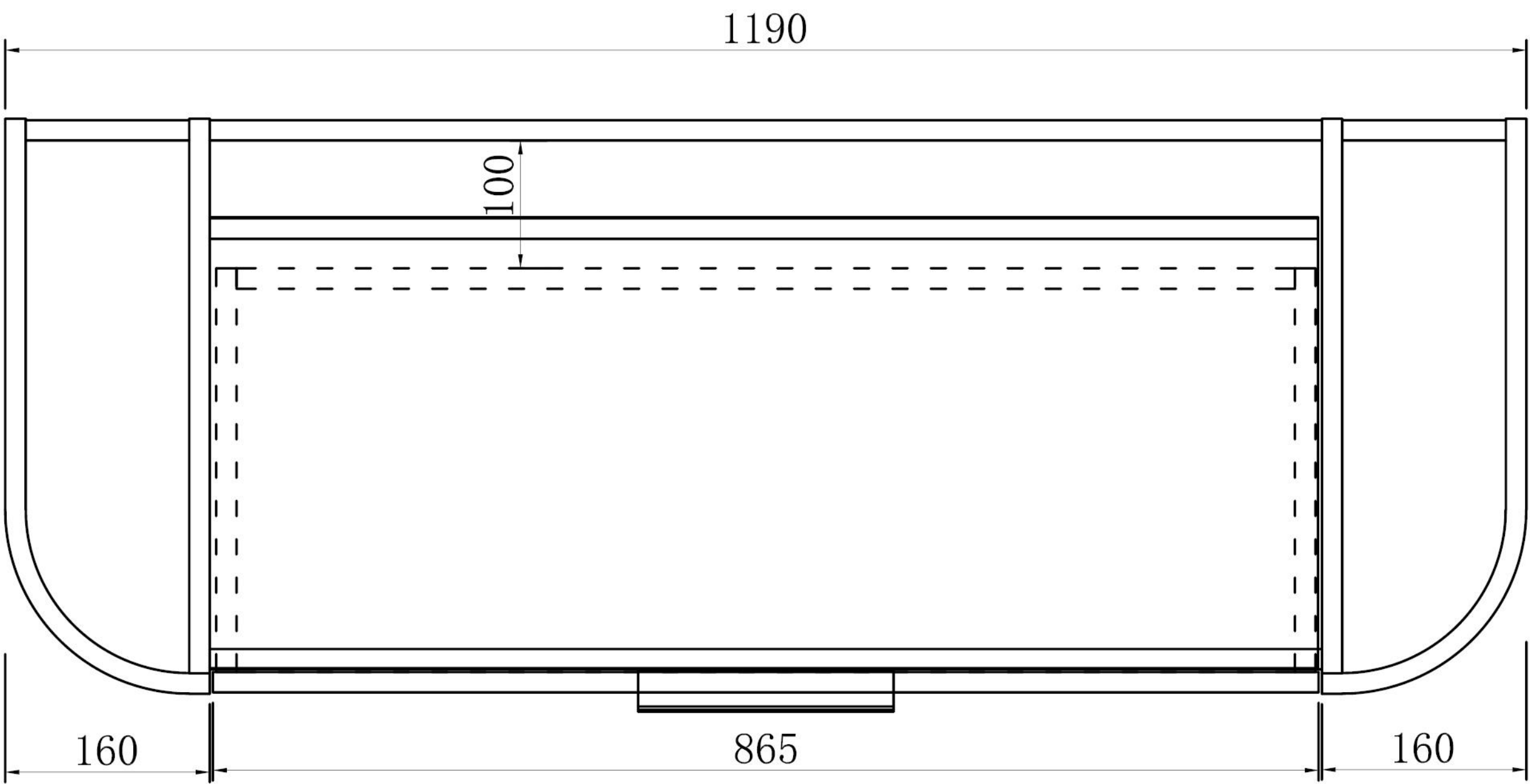
Top View
