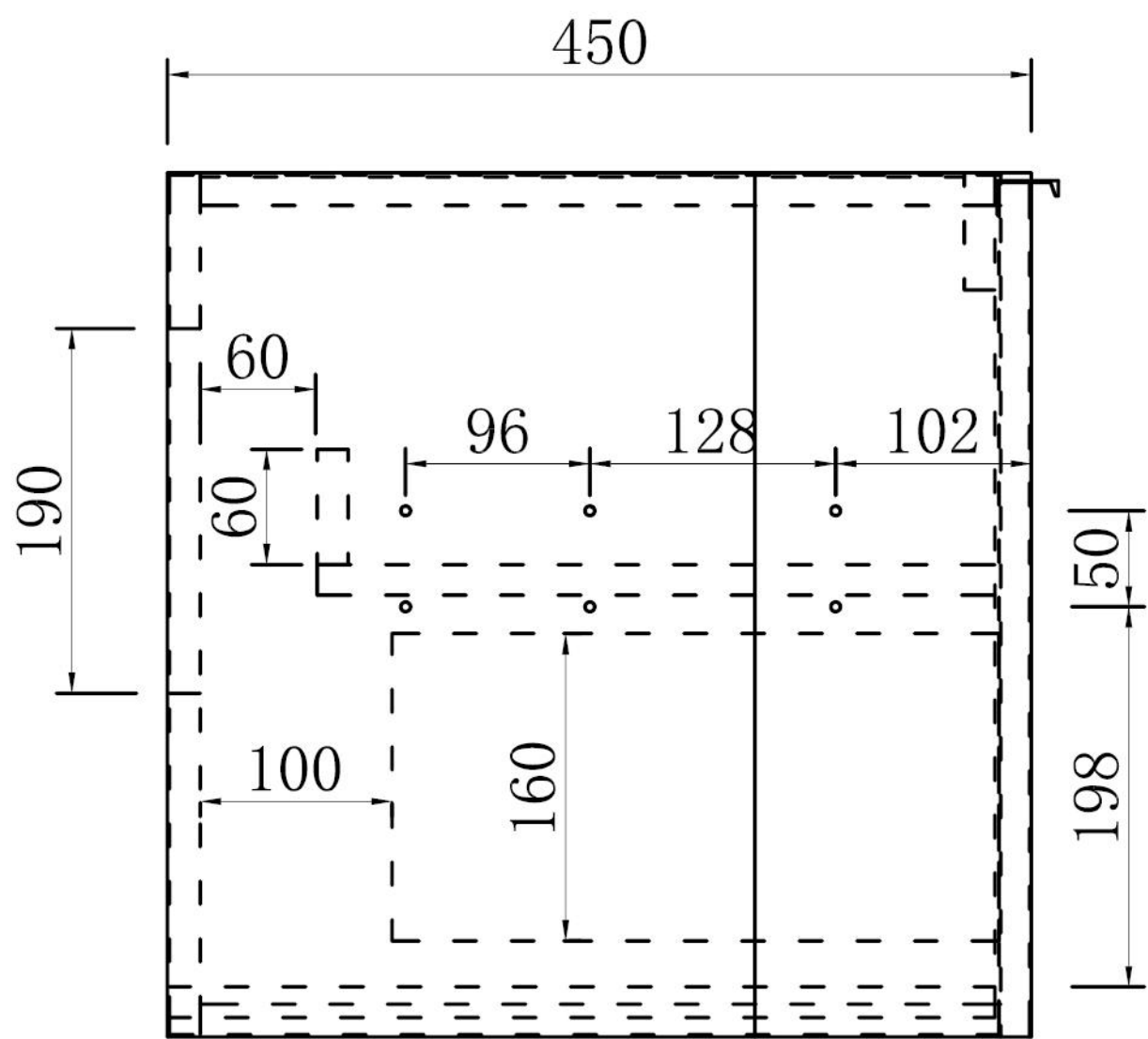
Side View
