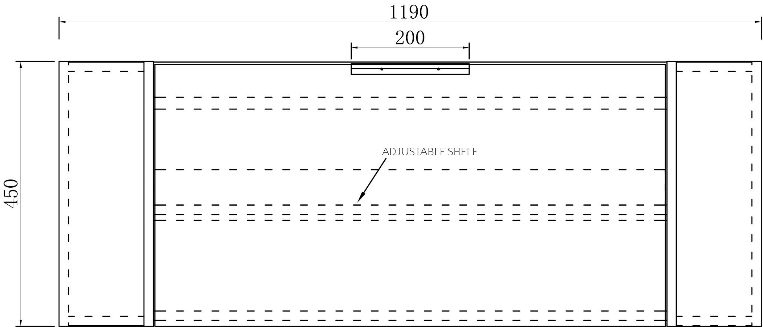
Front View
