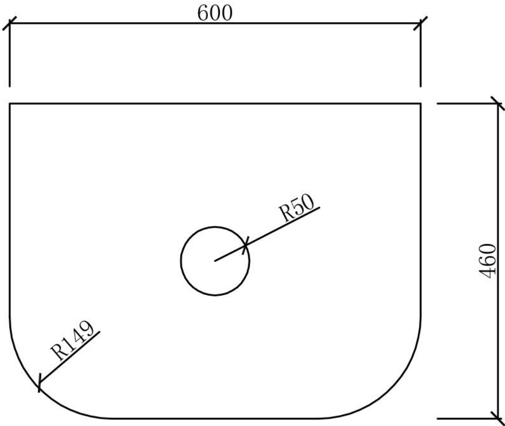
Front View
