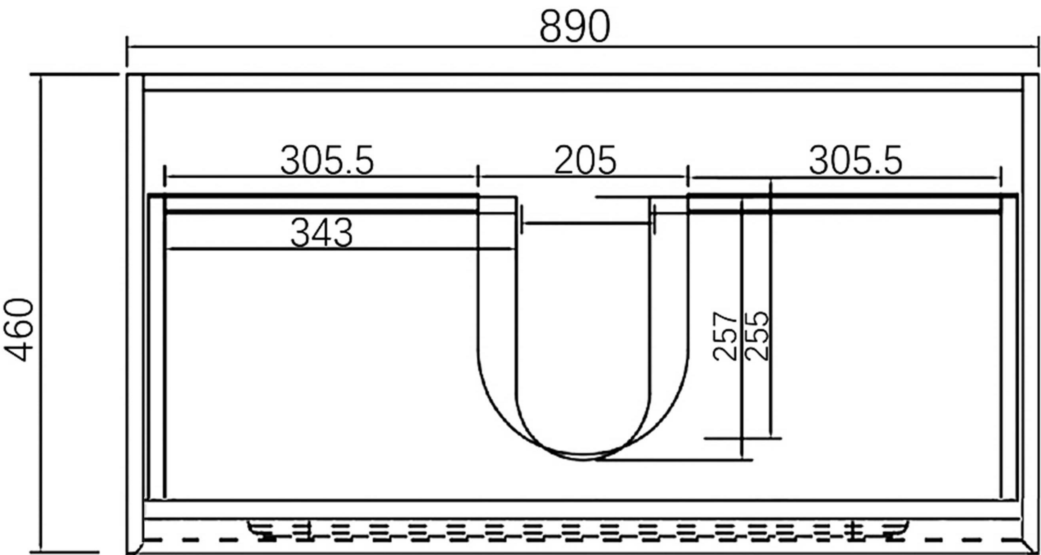
Top view
