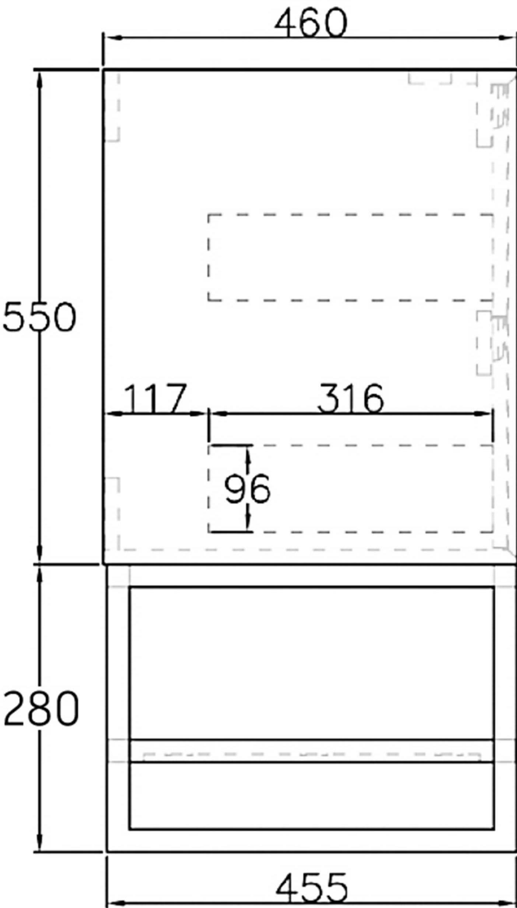
Side view
