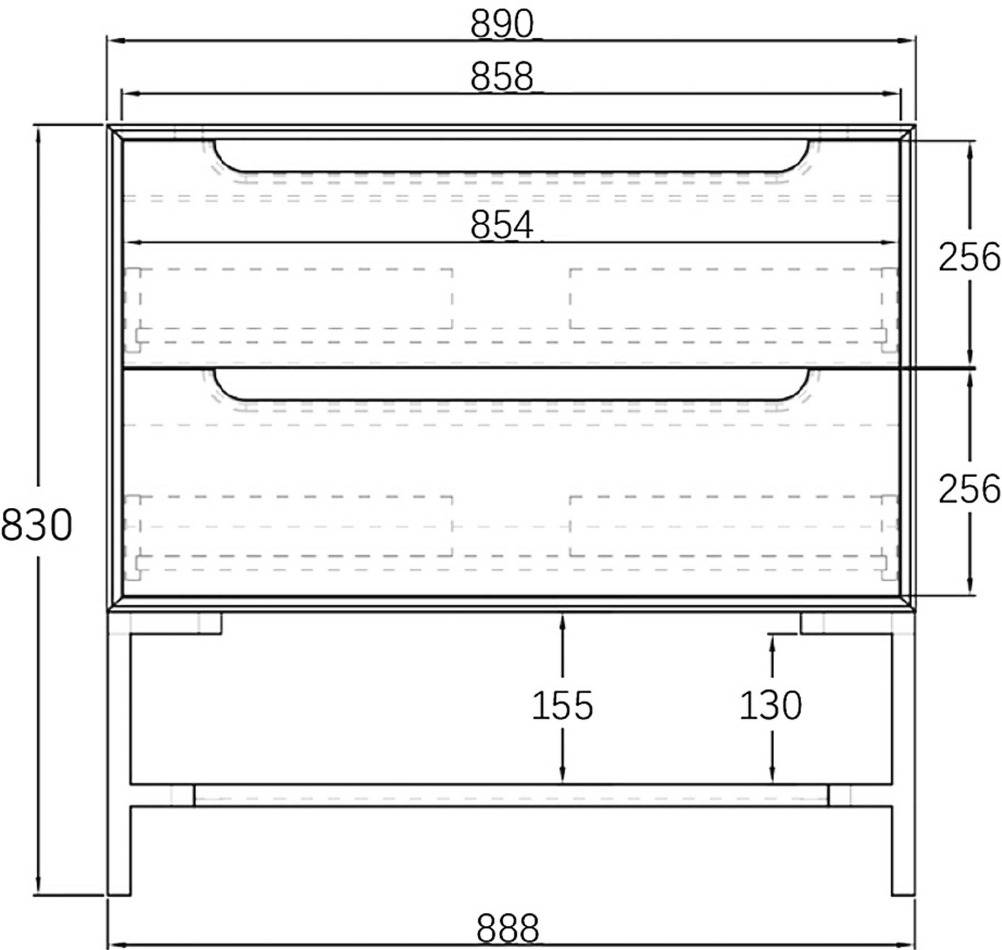
Front view
