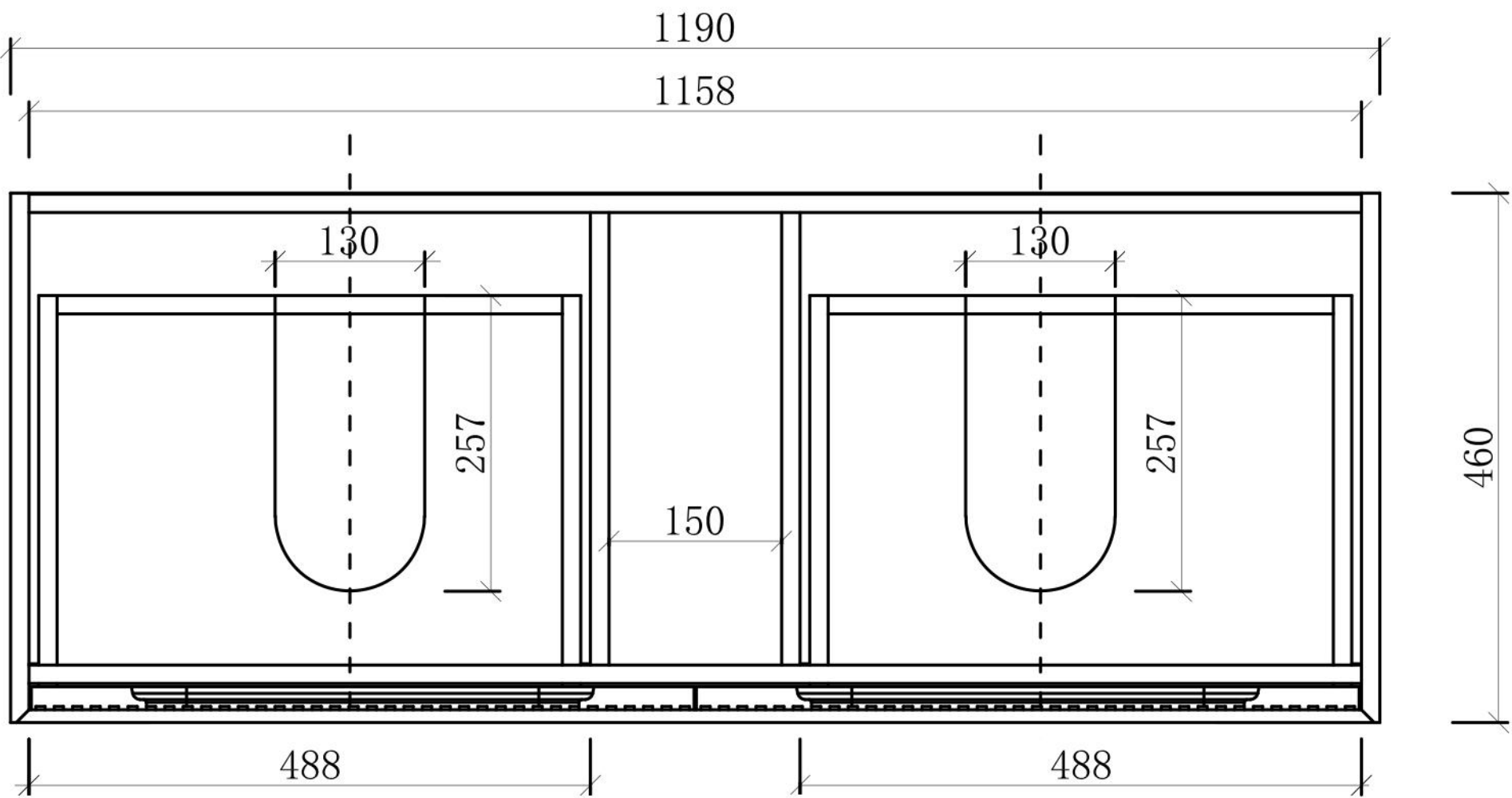
Top View
