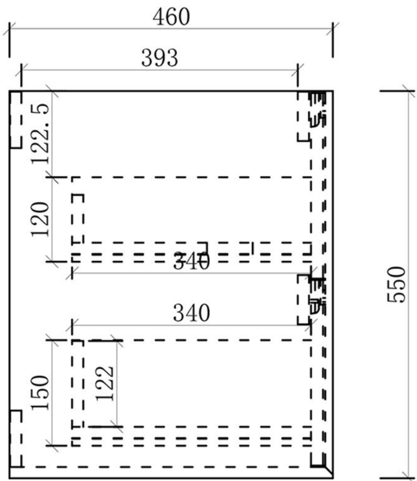
Side View
