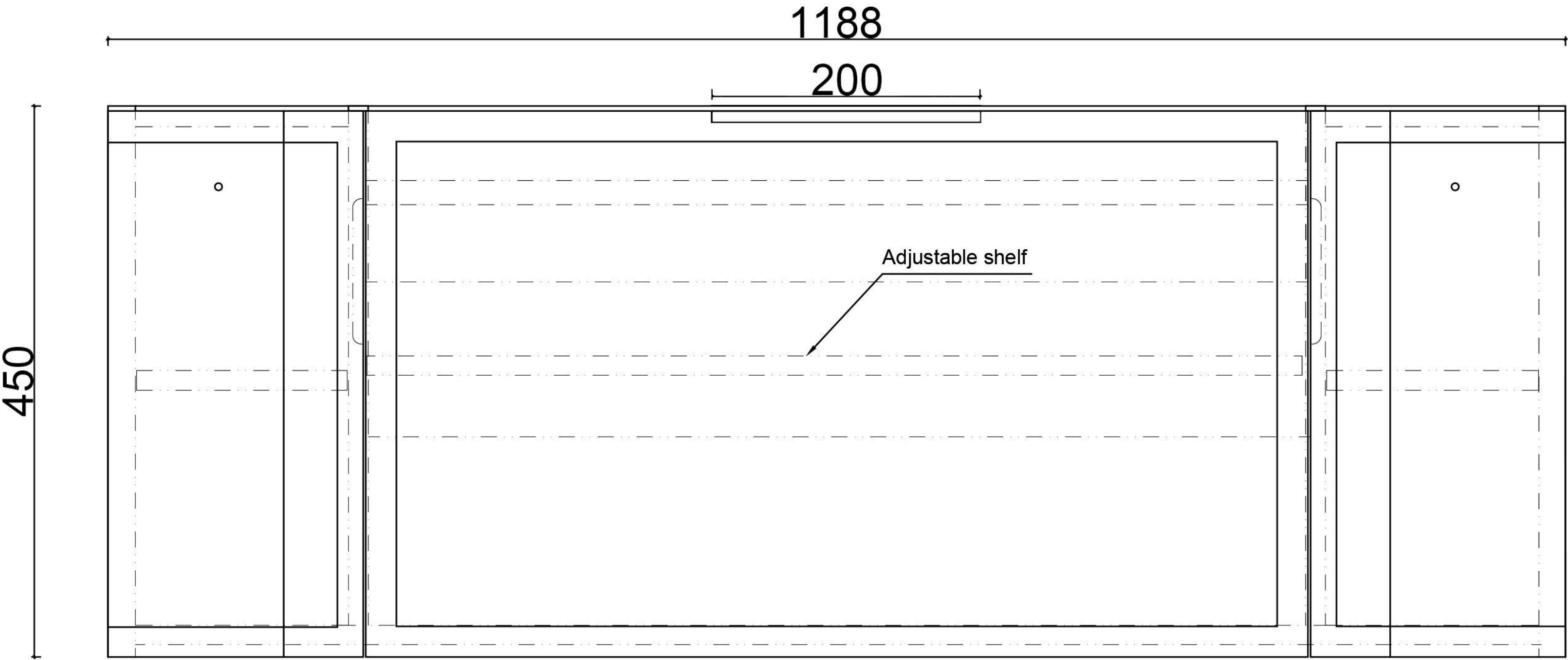
FRONT VIEW
