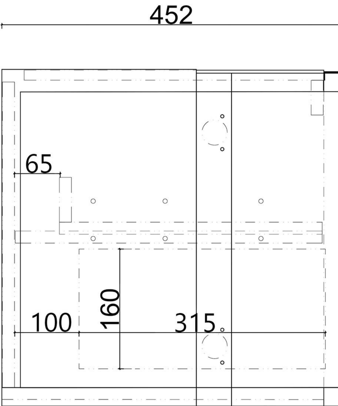
SIDE VIEW
