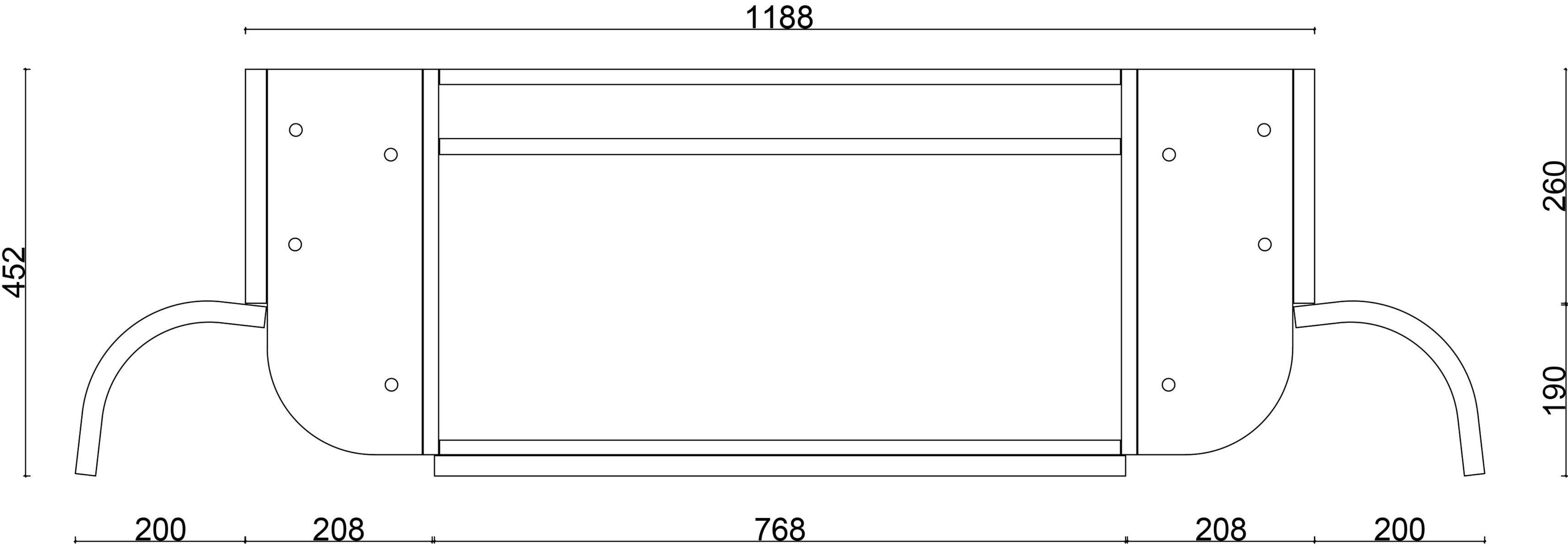
TOP VIEW
