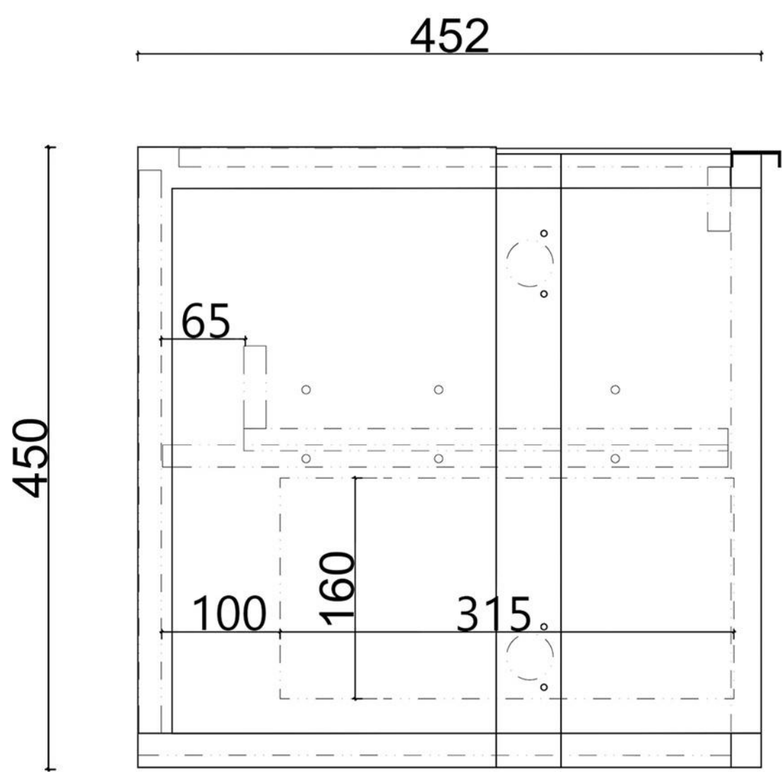
SIDE VIEW
