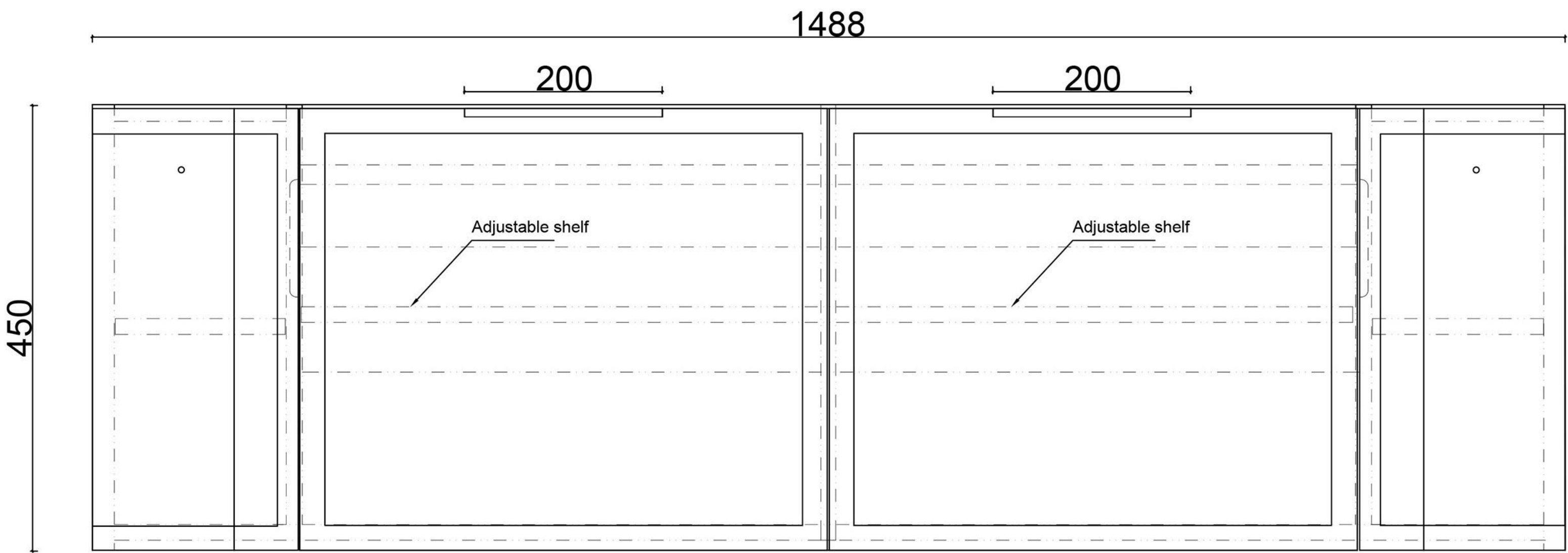
FRONT VIEW
