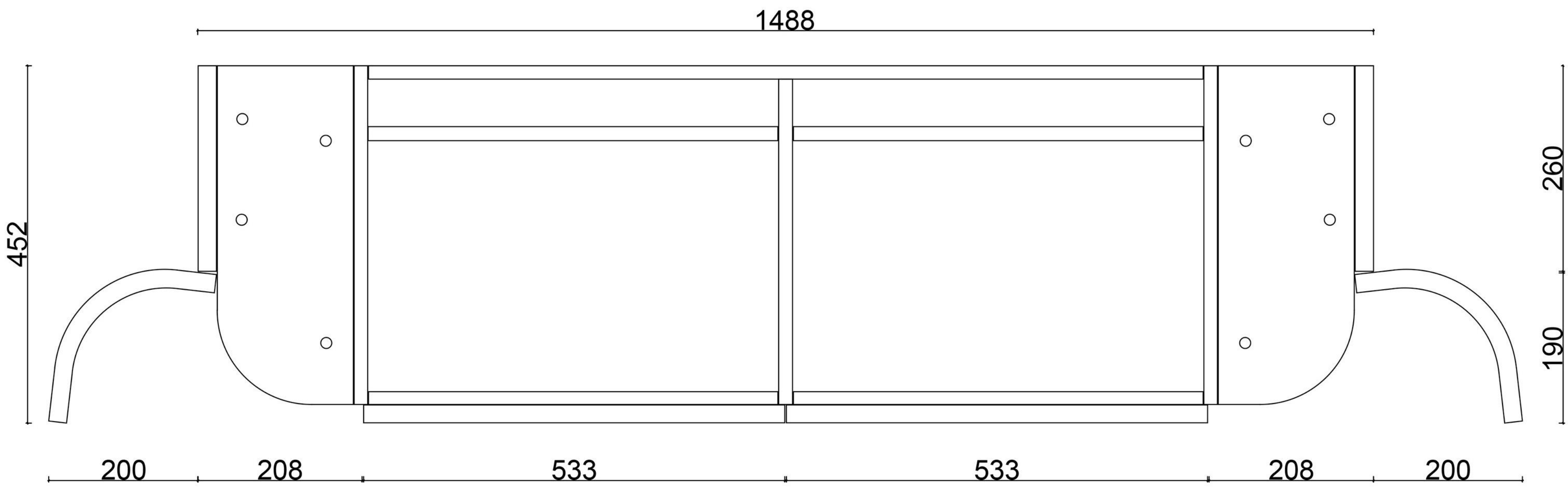
TOP VIEW
