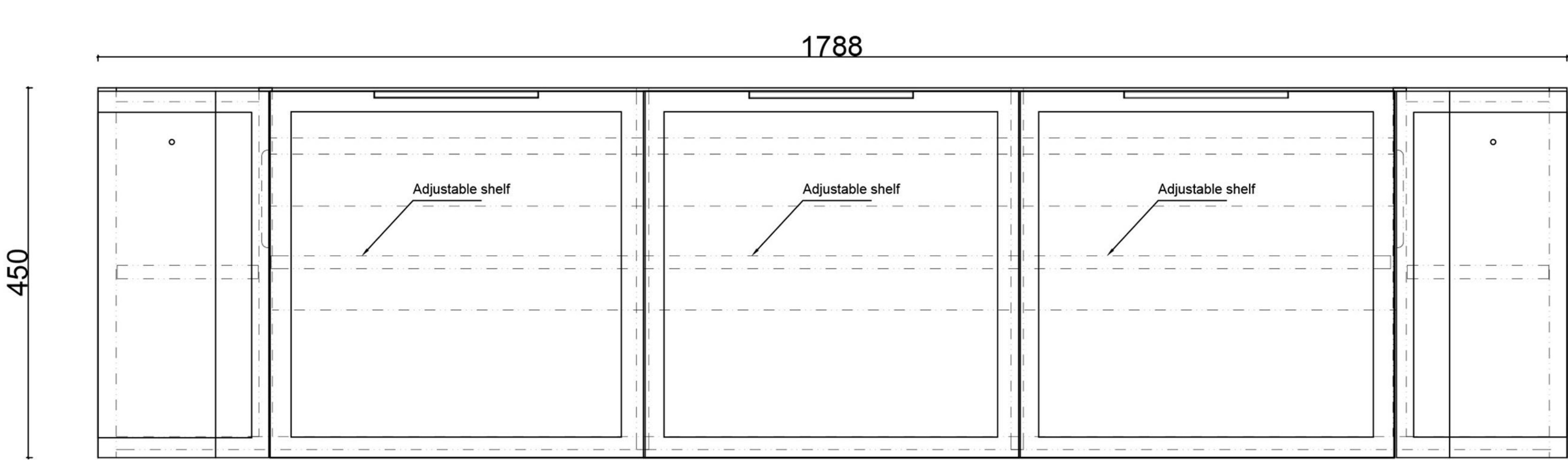
FRONT VIEW
