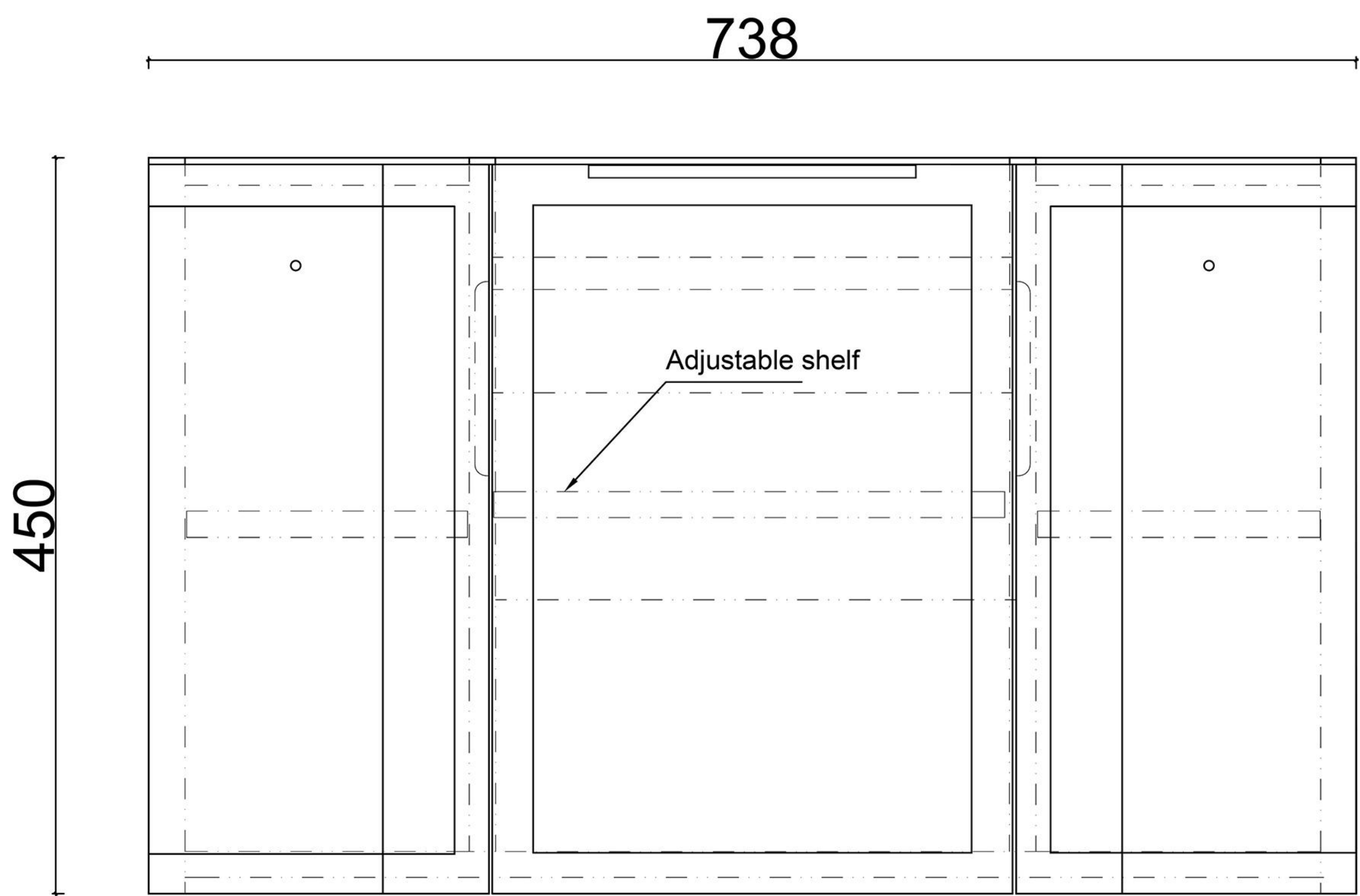
FRONT VIEW
