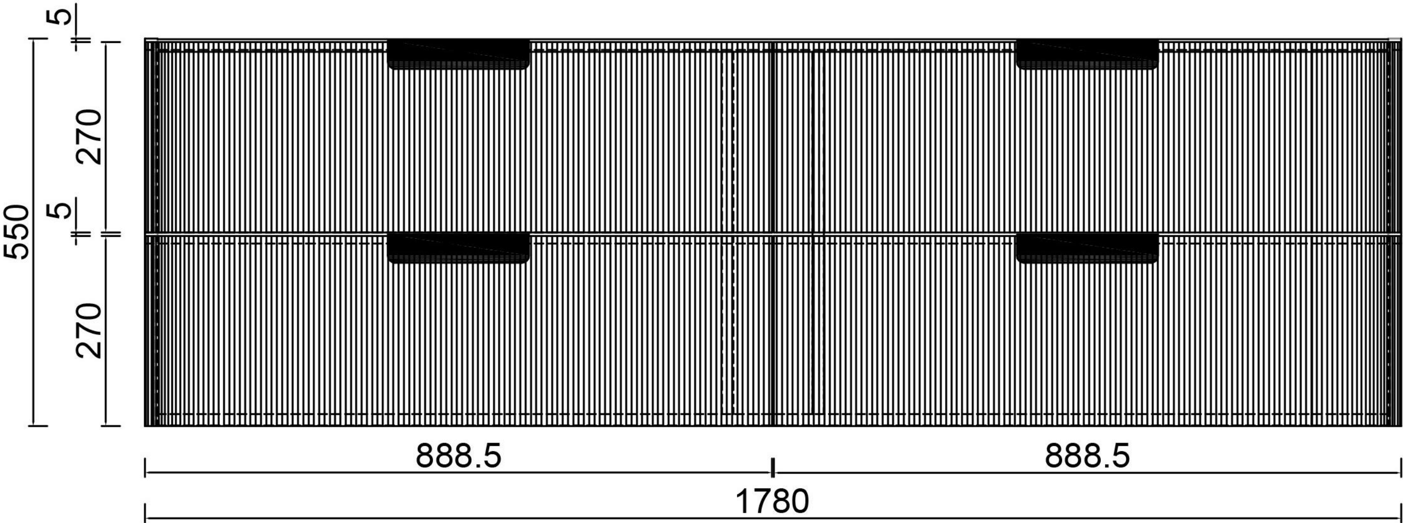
Front View
