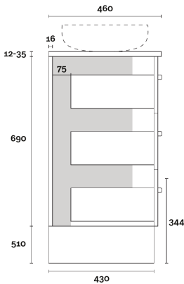
PROFILE Legs
