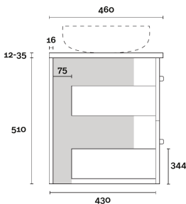
PROFILE Wallmount
