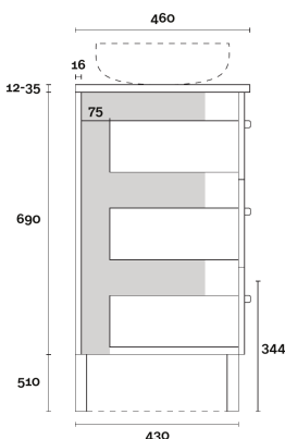
PROFILE Wallmount
