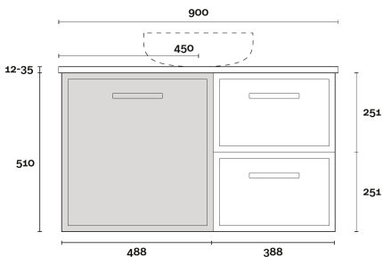
CONFIGURATION Wallmount
