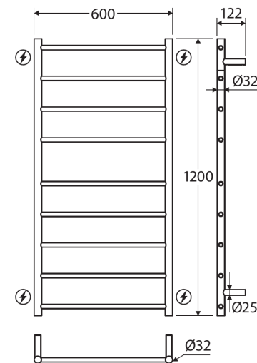
⚡ Wiring Positions
