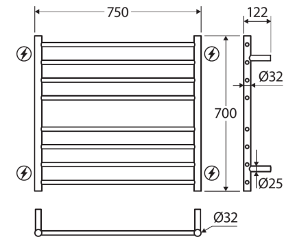
⚡ Wiring Positions
