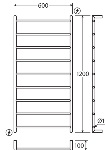
⚡ Wiring Positions
