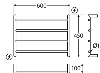
⚡ Wiring Positions
