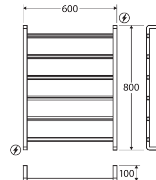
⚡ Wiring Positions
