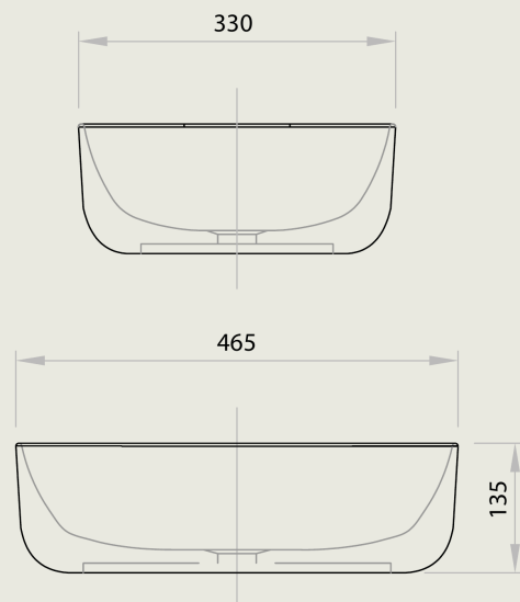
SIDE VIEWS
