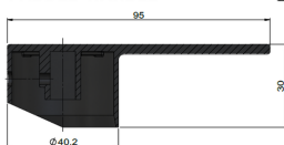
PADDLE HANDLE
