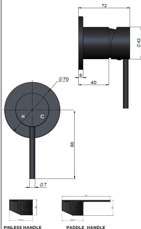
PINLESS HANDLE
