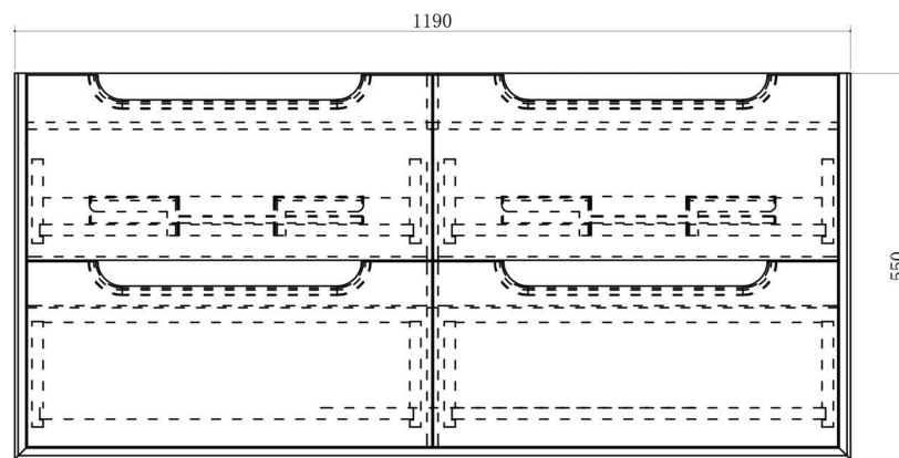
Front View
