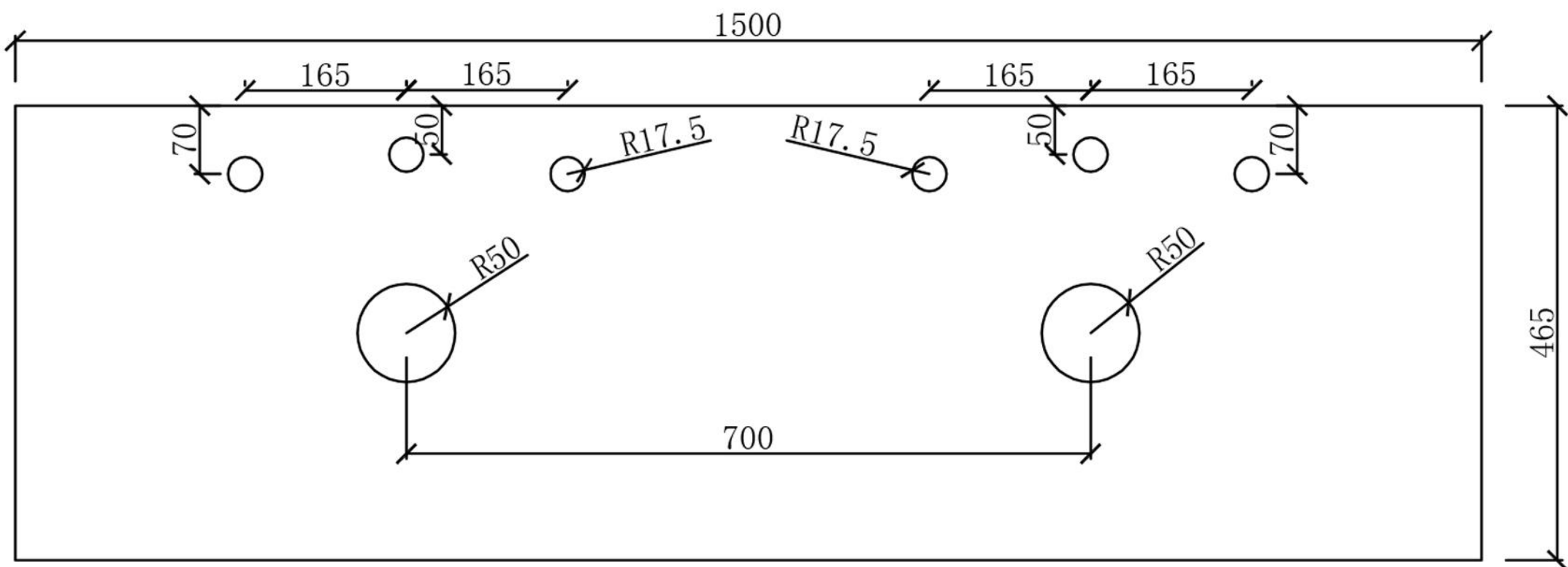
Back View Pre Semi-Drilling Taphole
