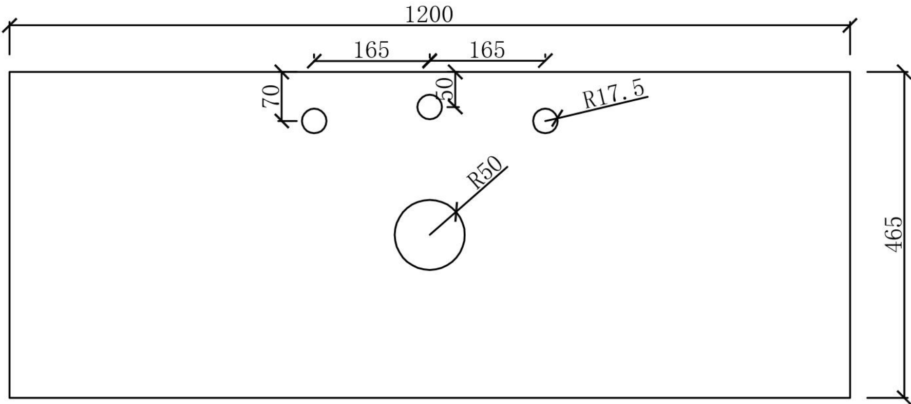
Back View Pre Semi-Drilling Taphole
