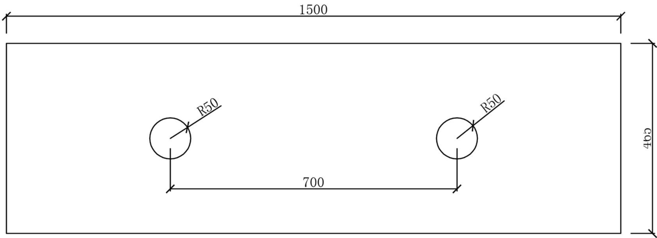
Front View
