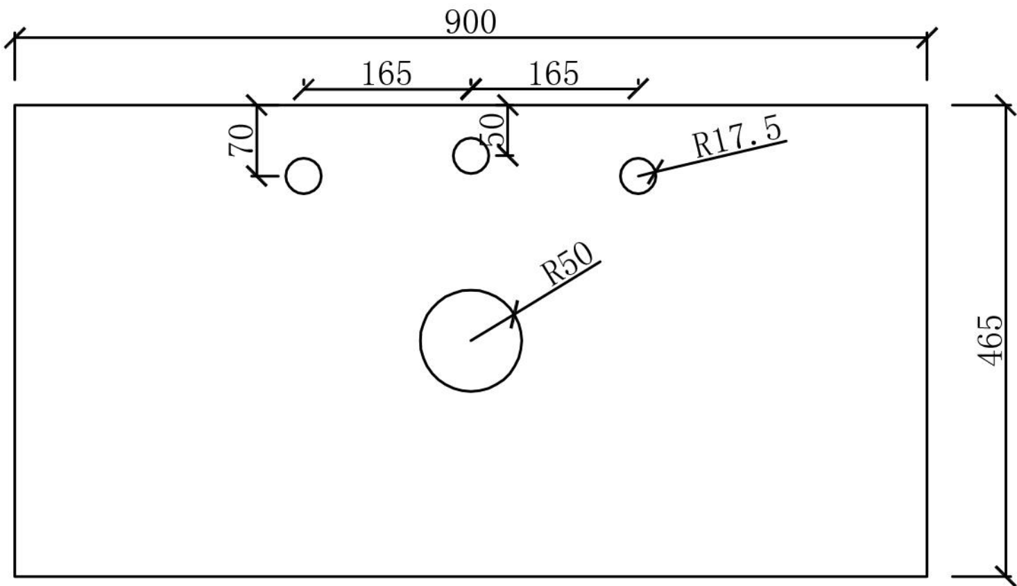
Back View Pre Semi-Drilling Taphole
