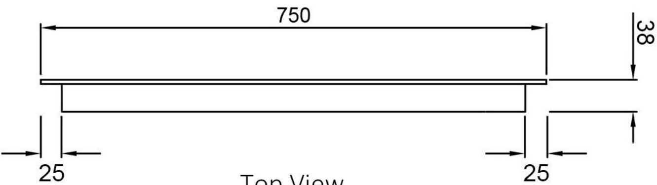
Top View
