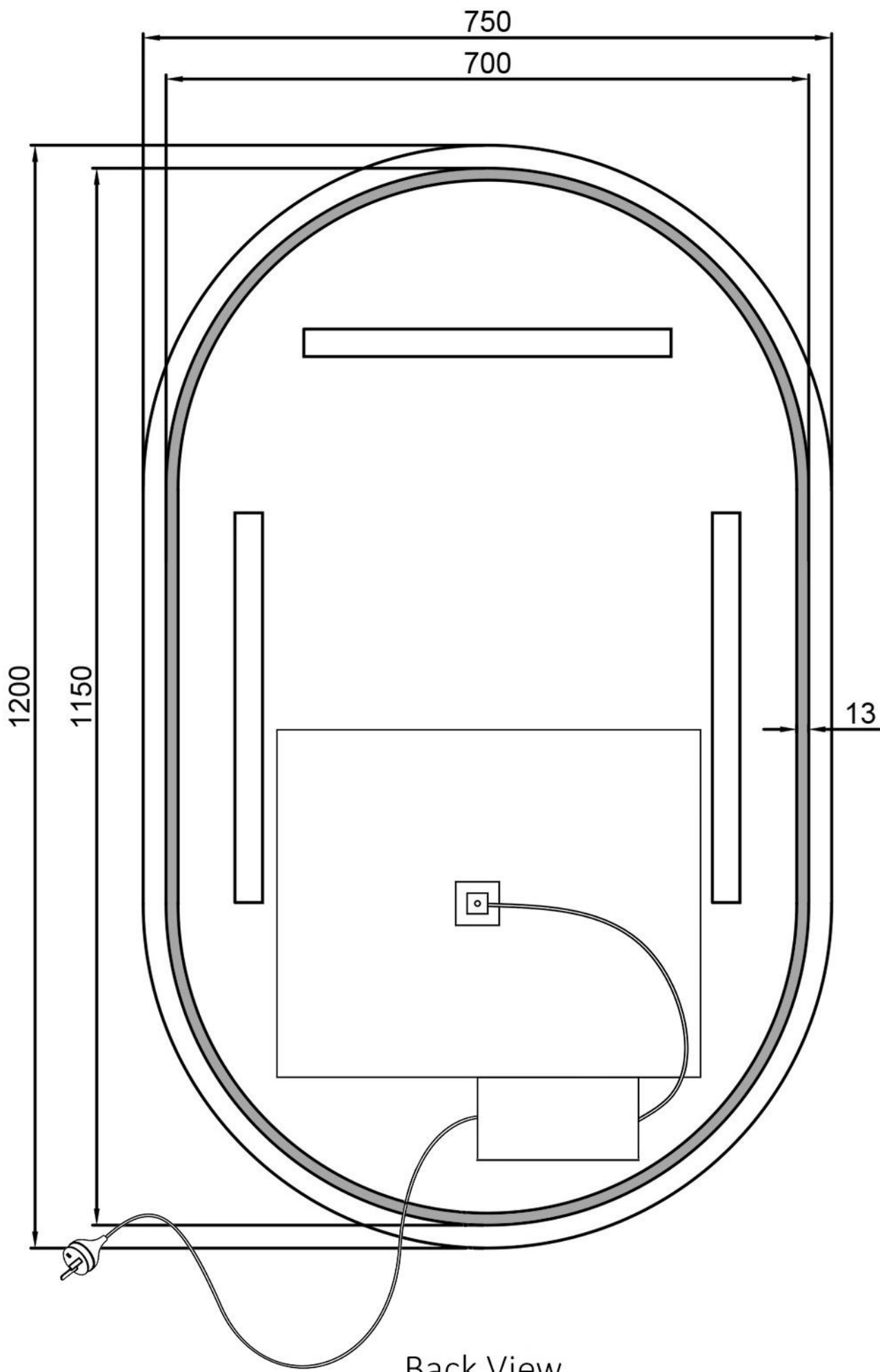
Back View
