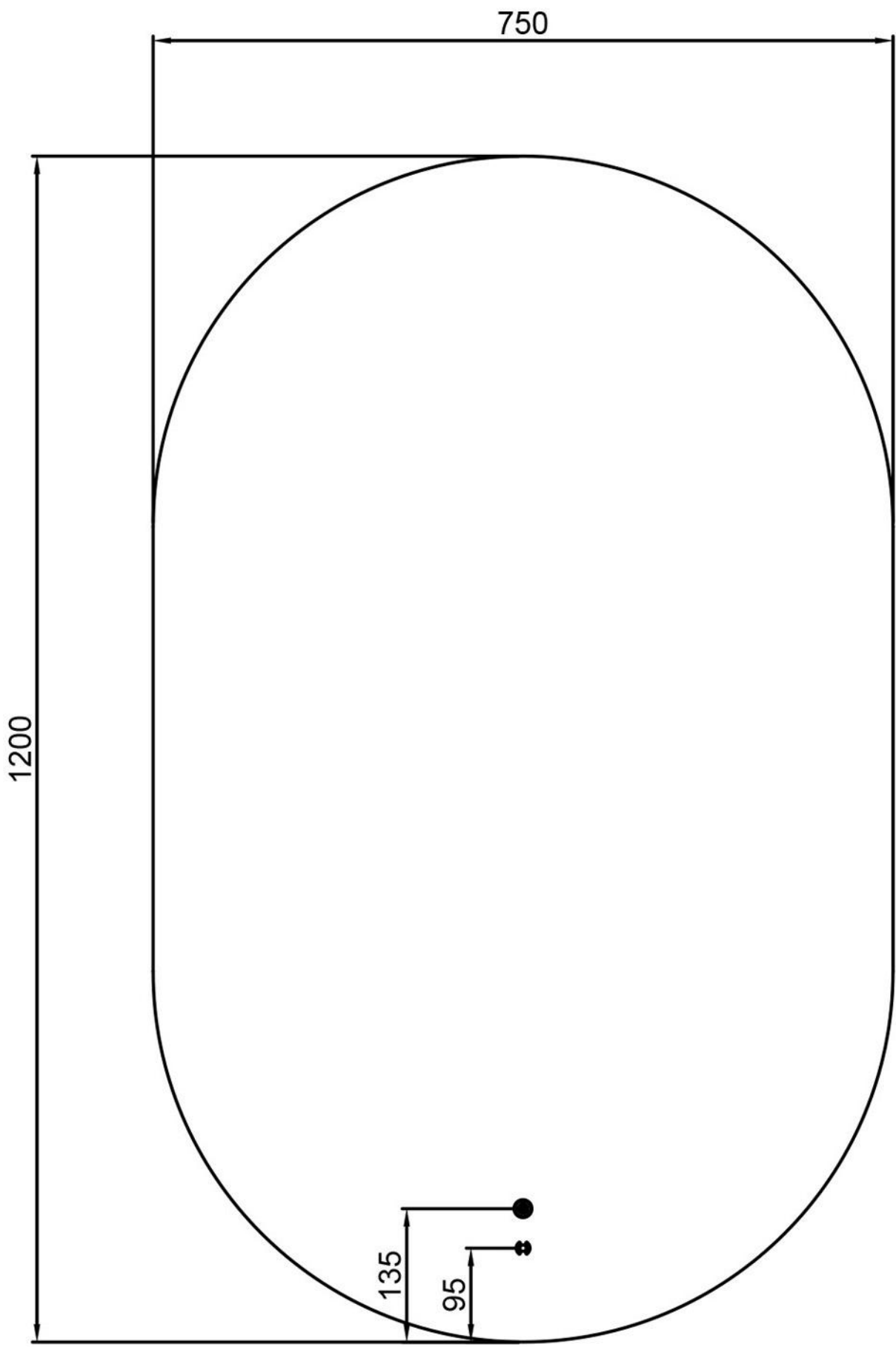
Front View
