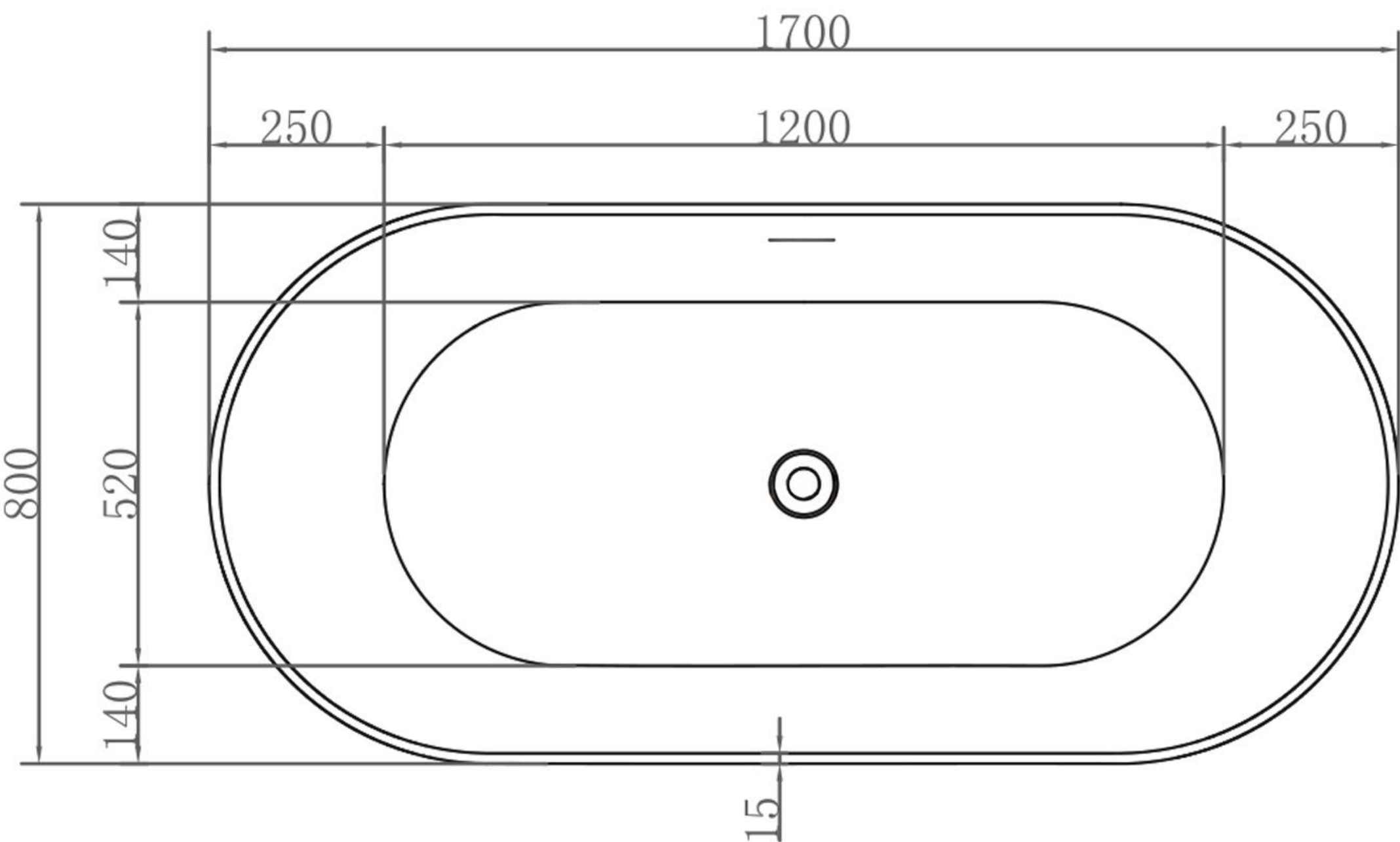
Top View
