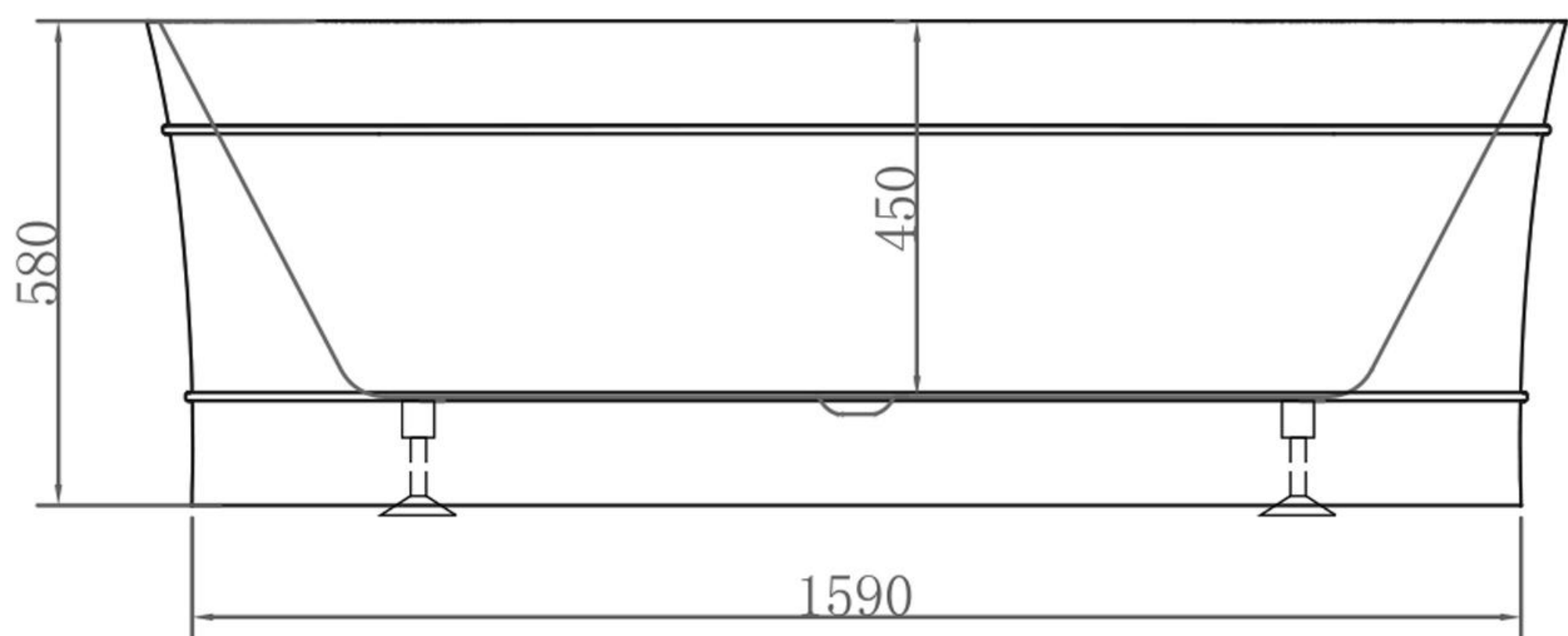
Front View
