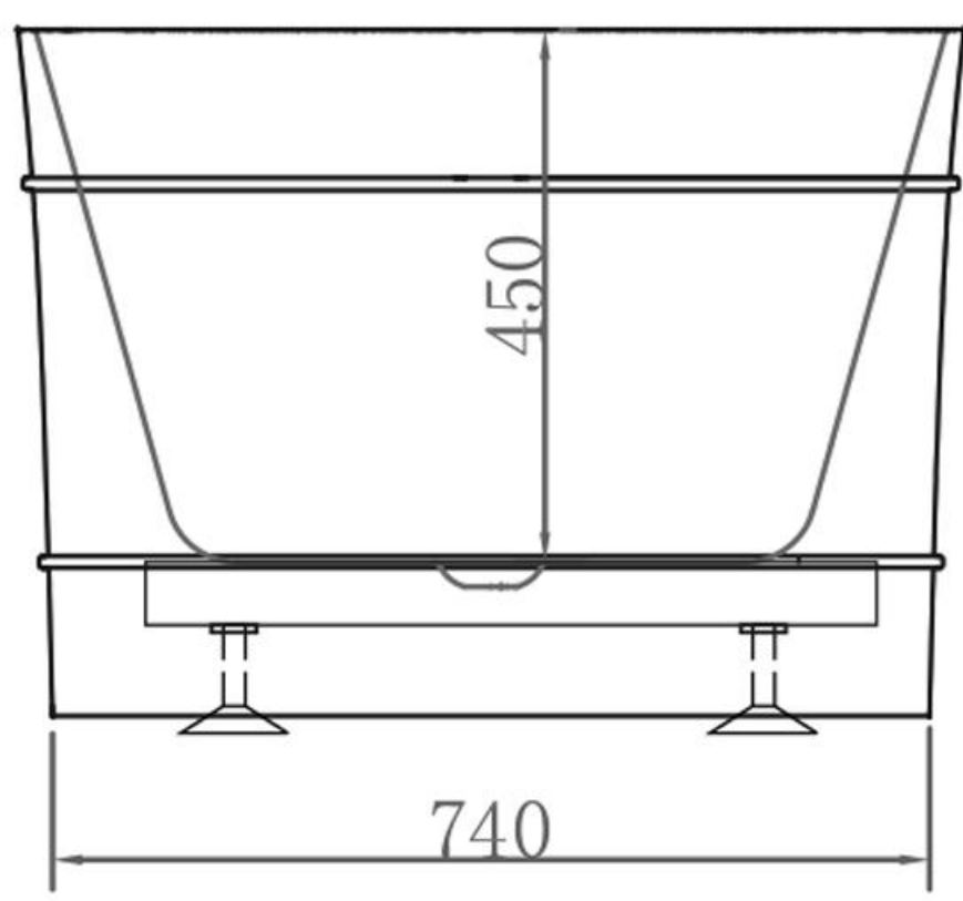
Side View
