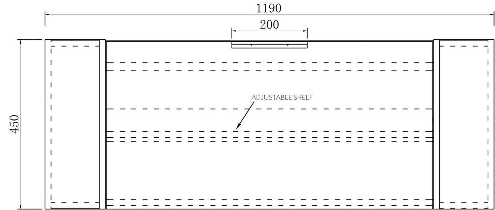
Front View
