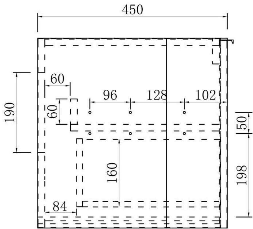
Side View
