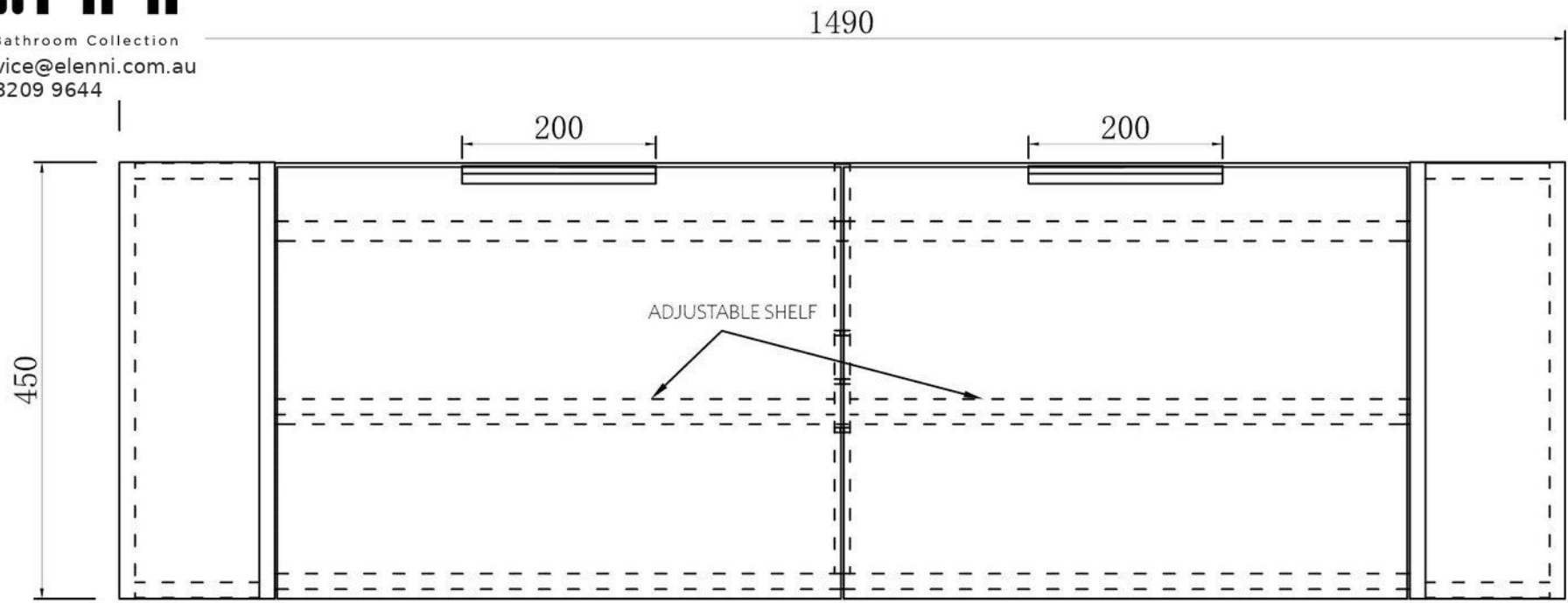
Front View
