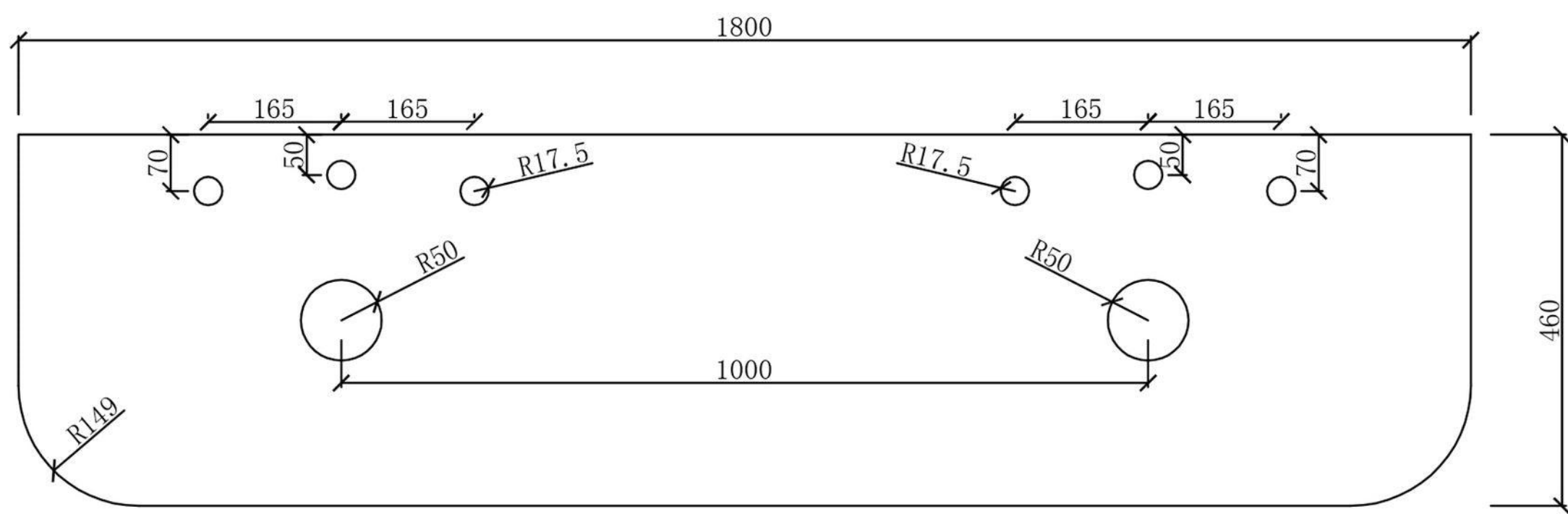
Back View Pre Semi-Drilling Taphole
