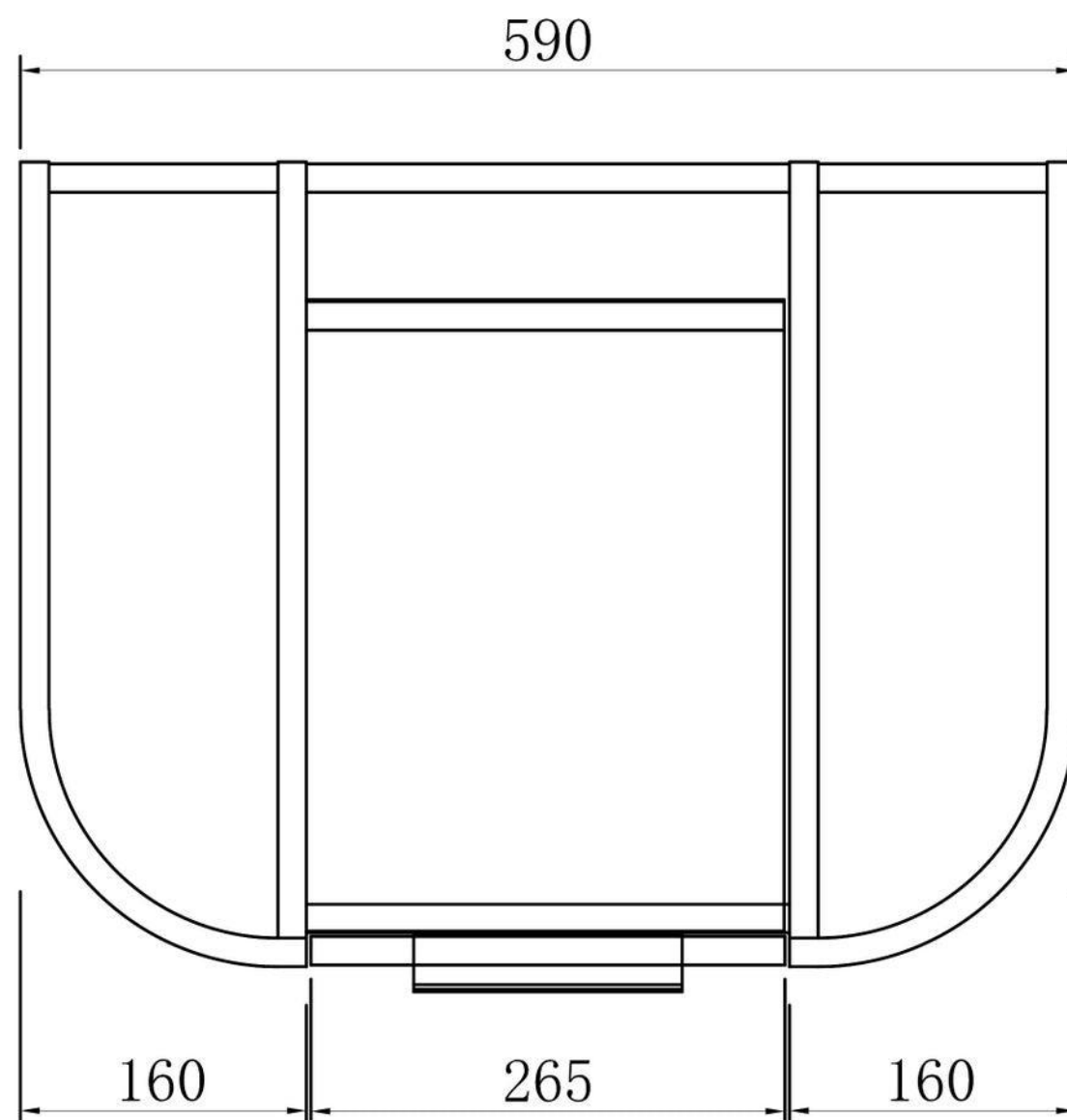
Top View
