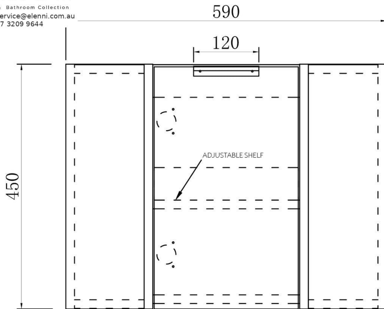
Front View
