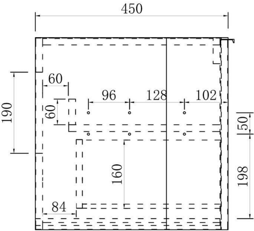
Side View
