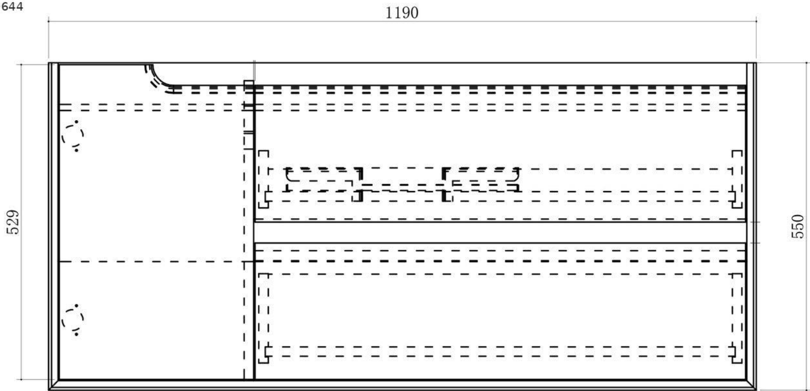
Front View
