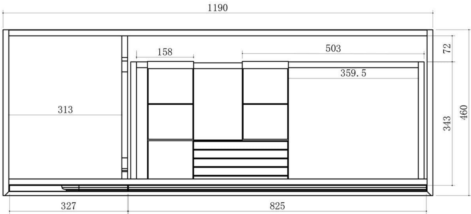
Top View
