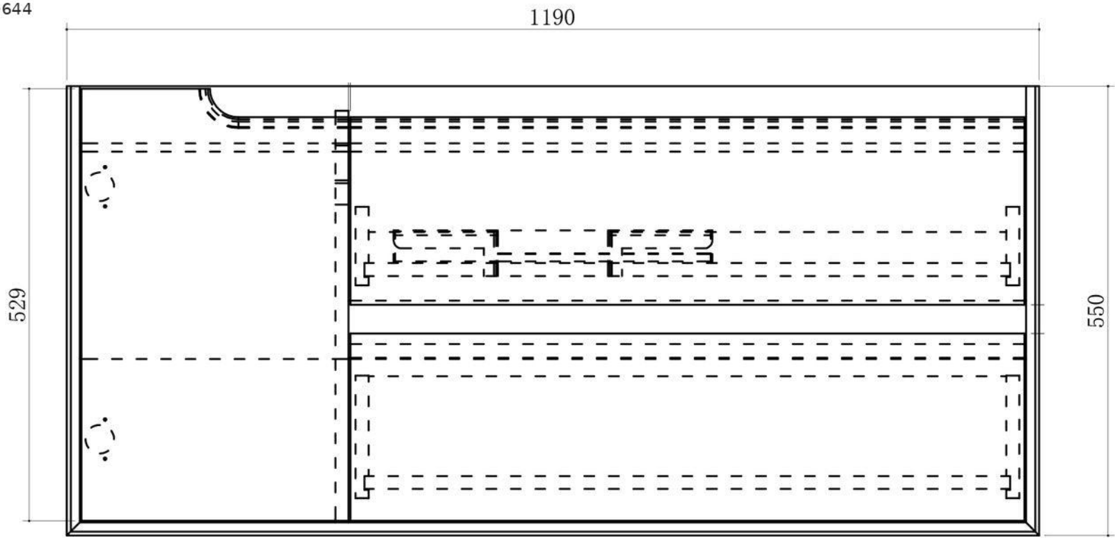
Front View
