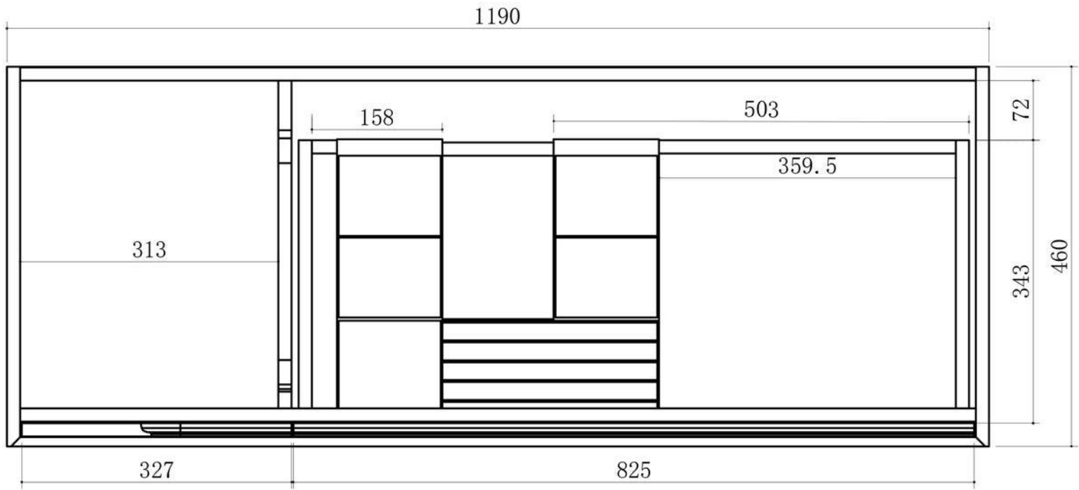
Top View
