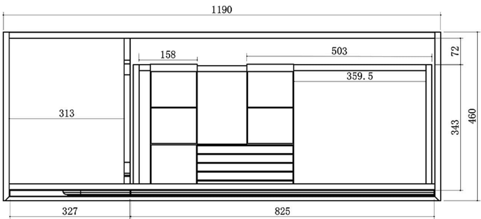
Top View
