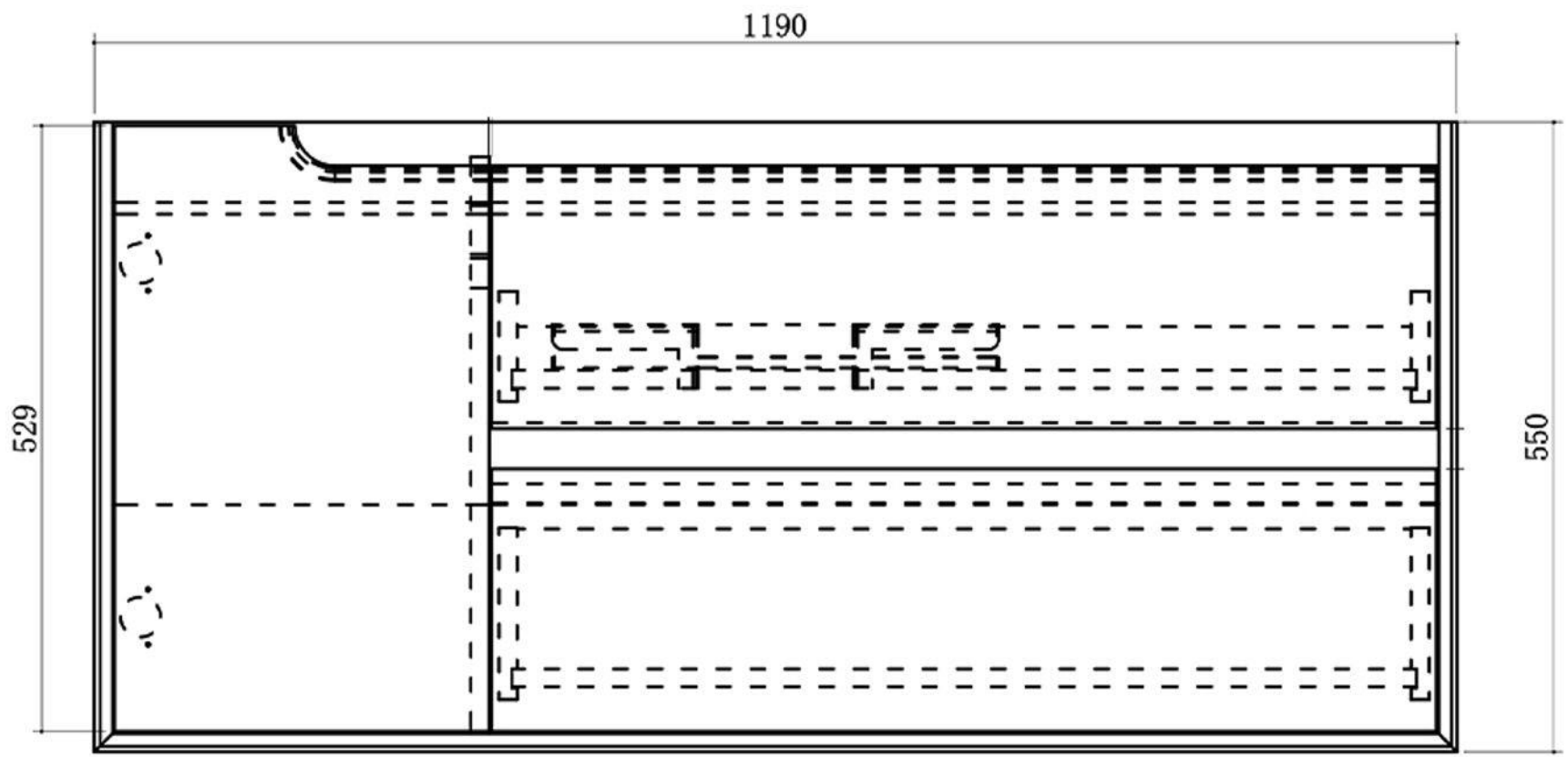
Front View
