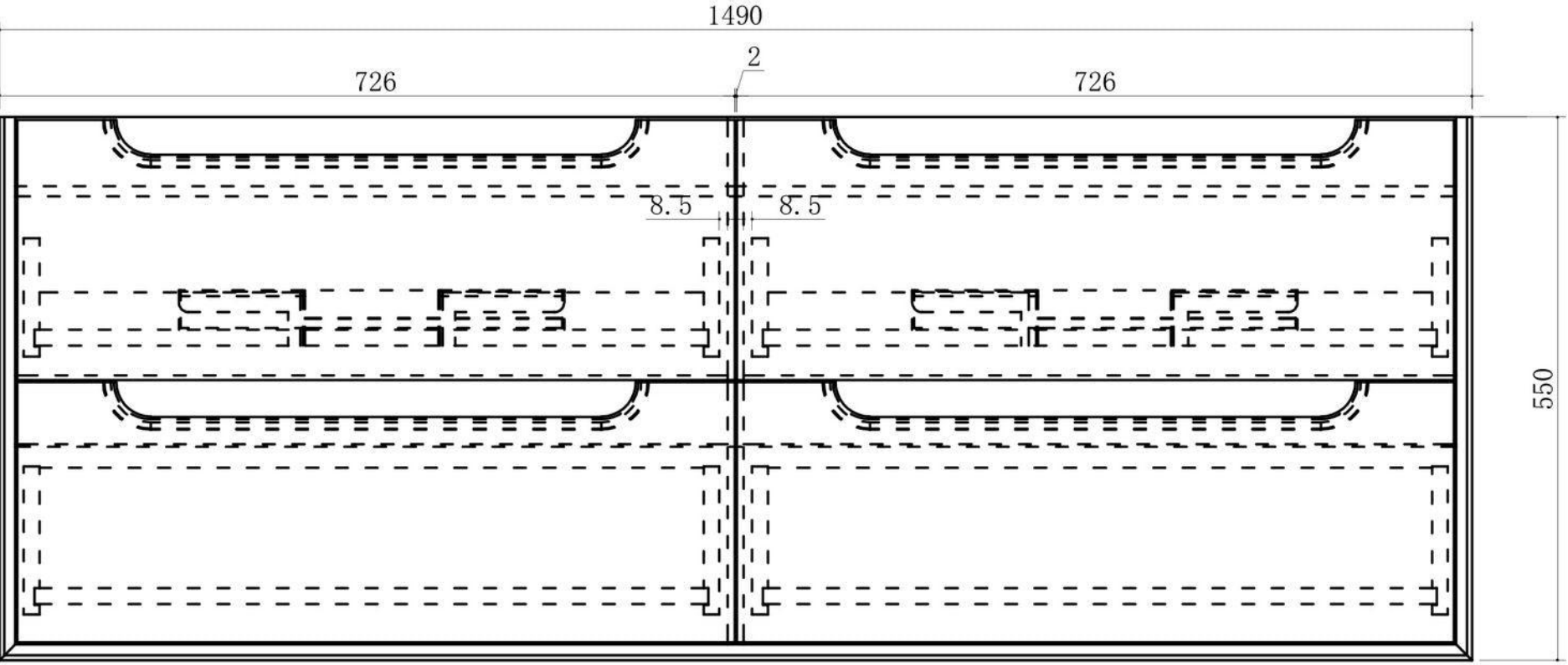
Front View
