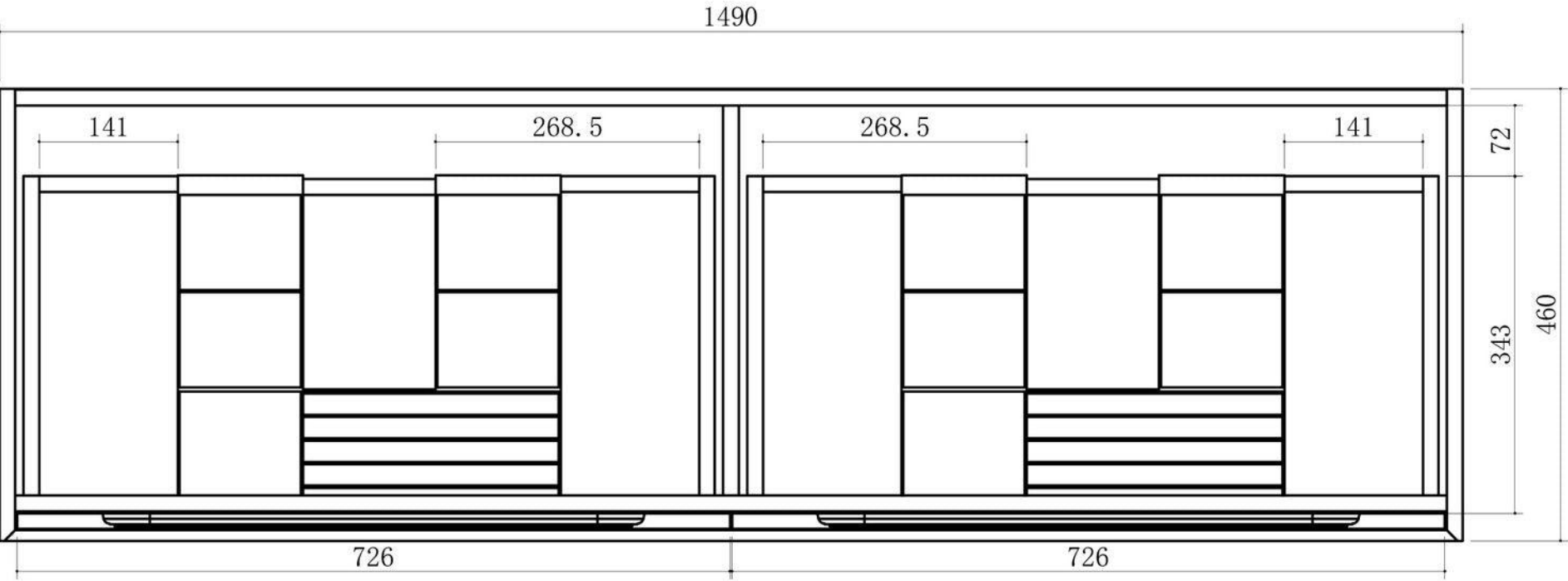
Top View
