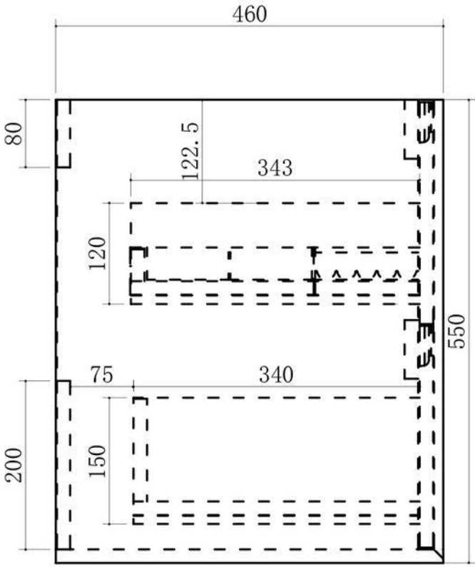
Side View
