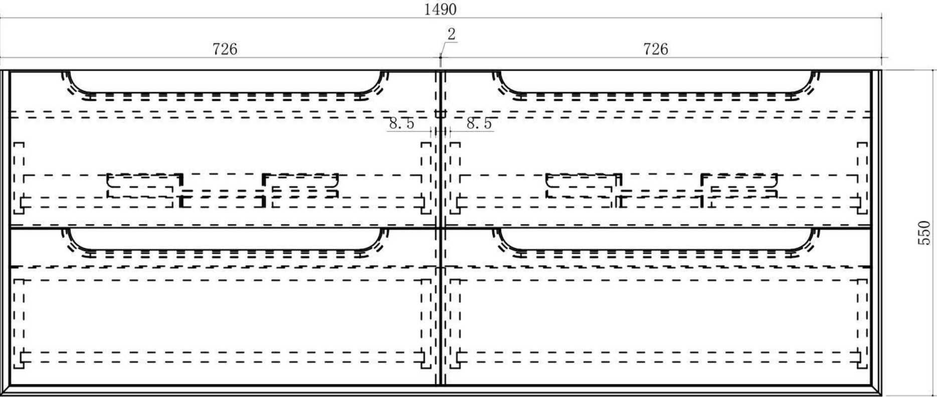
Front View
