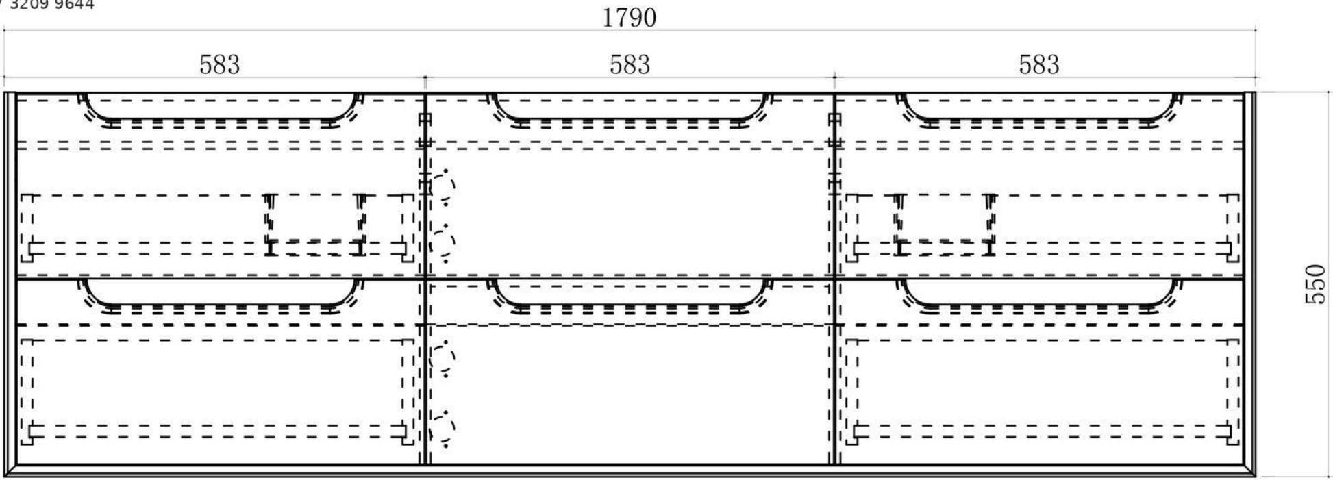
Front View
