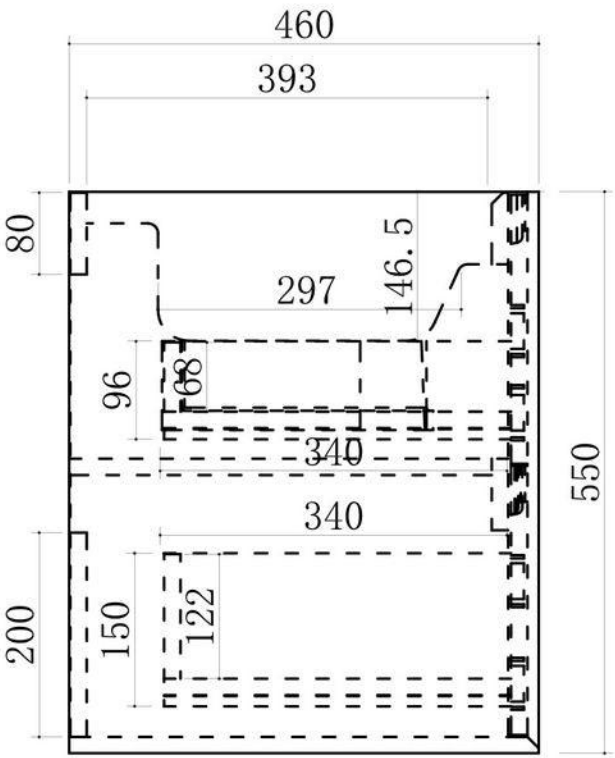
Side View
