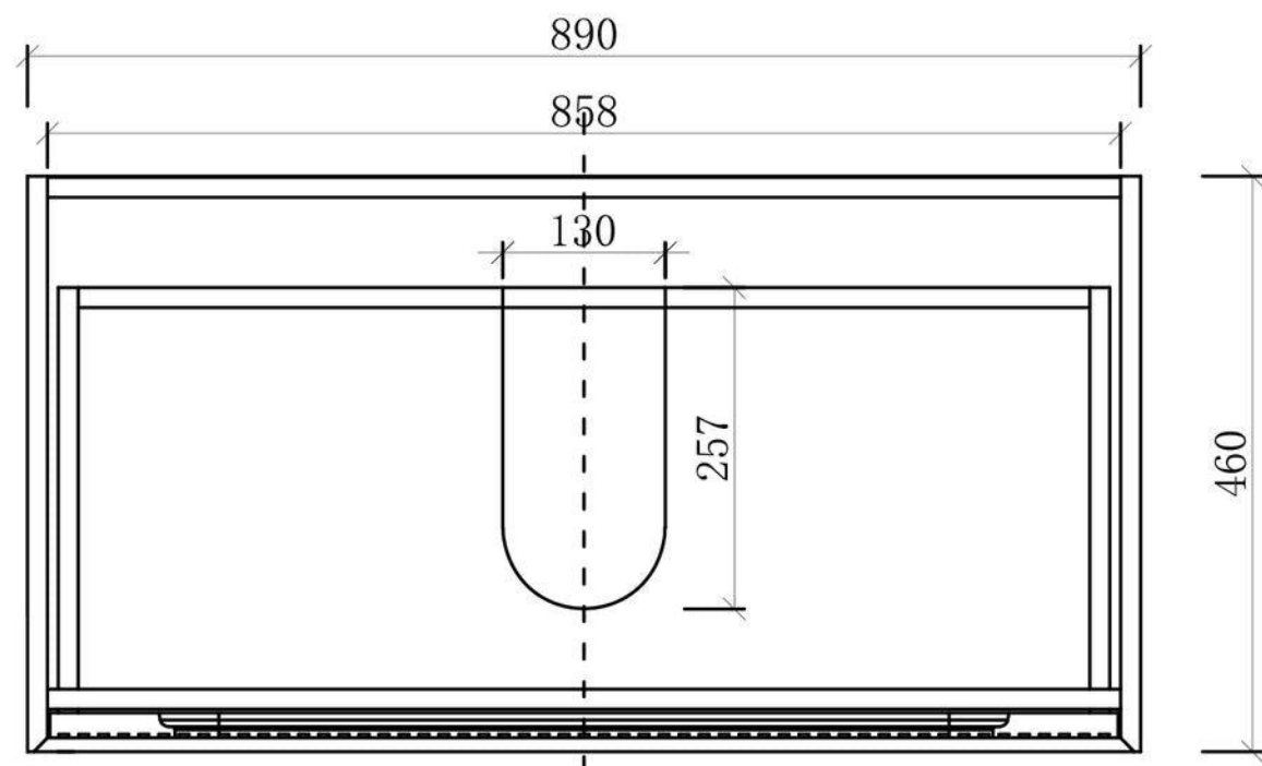
Top View
