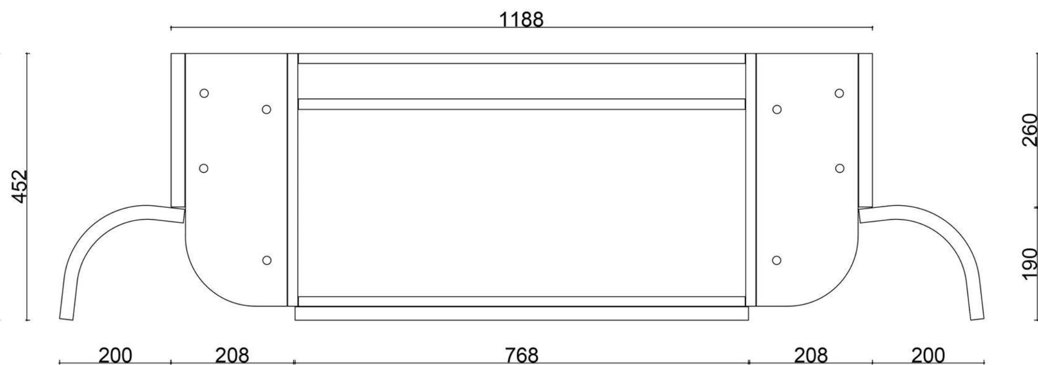
TOP VIEW
