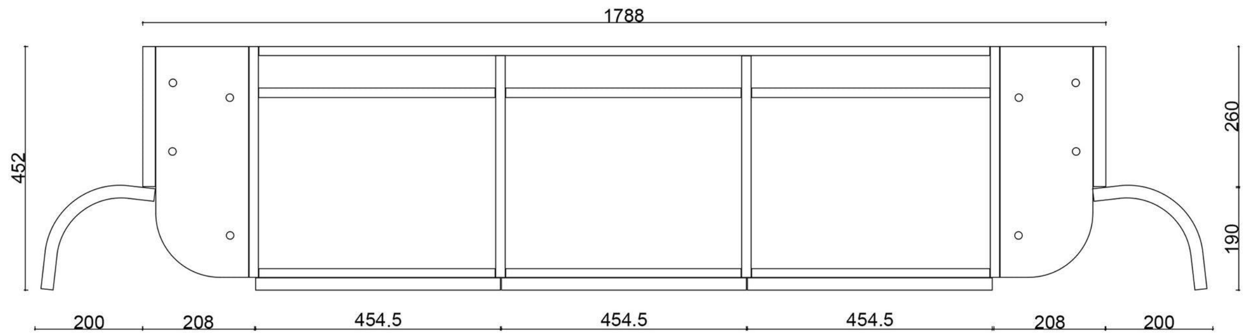
TOP VIEW
