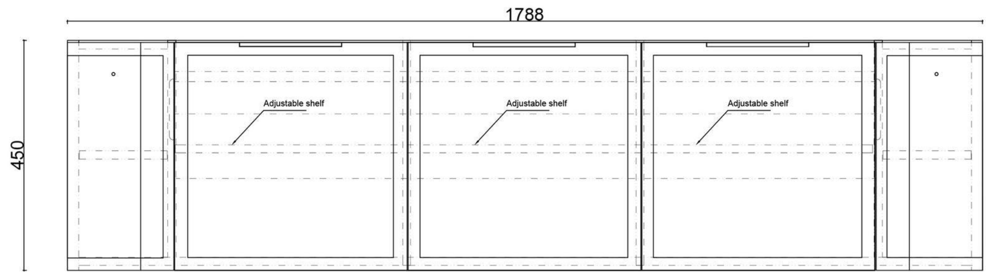
FRONT VIEW
