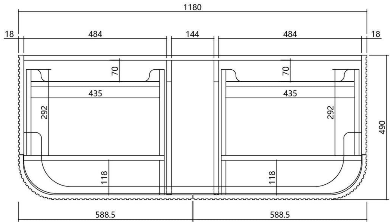
Top View
