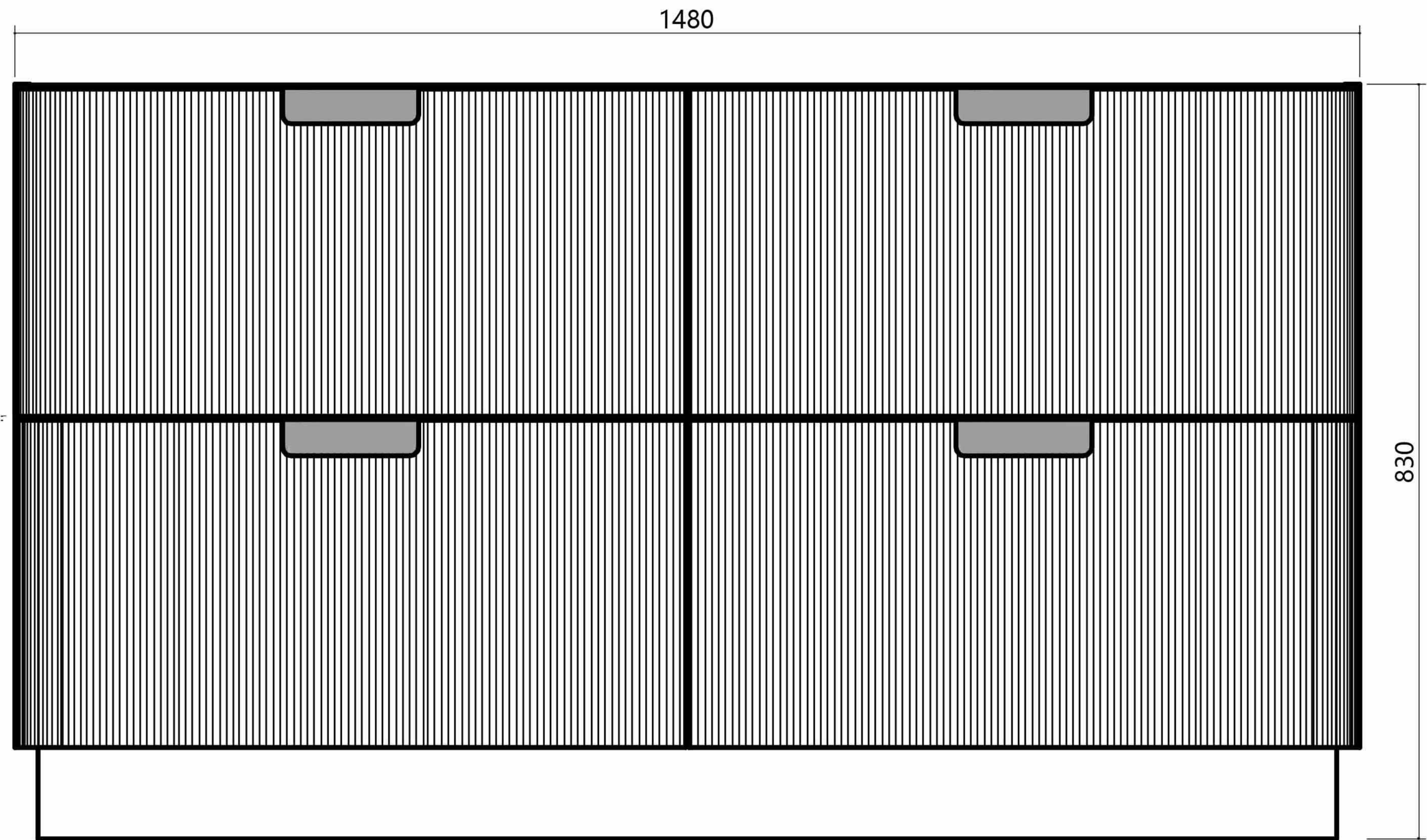
Front View
