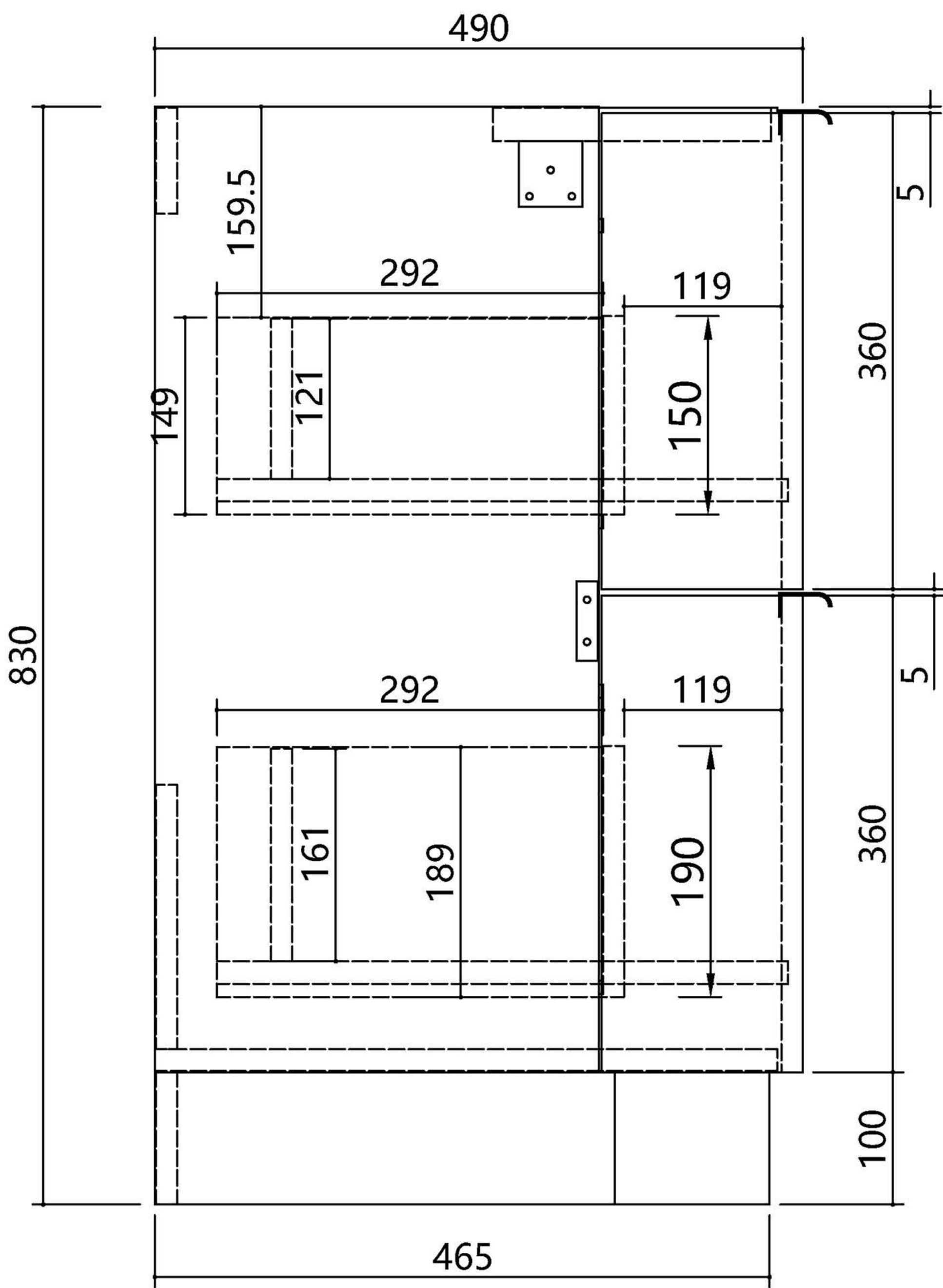
Side View
