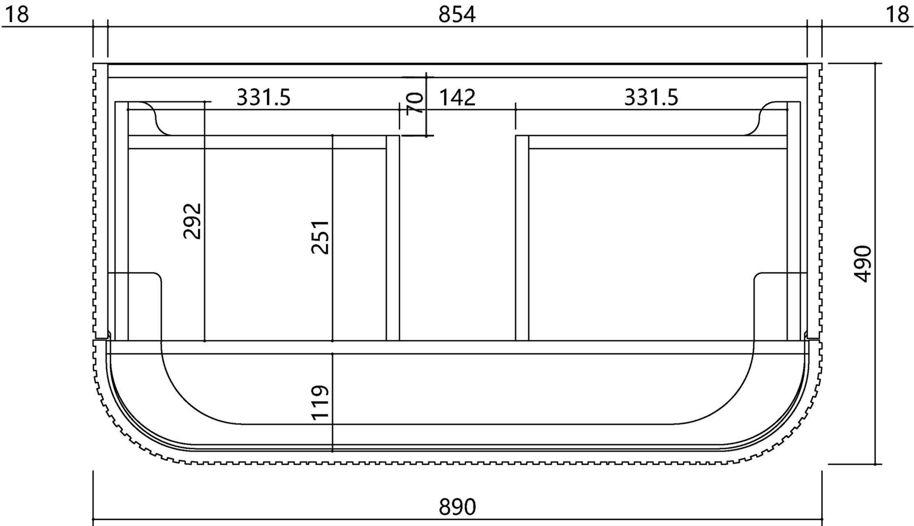
Top View
