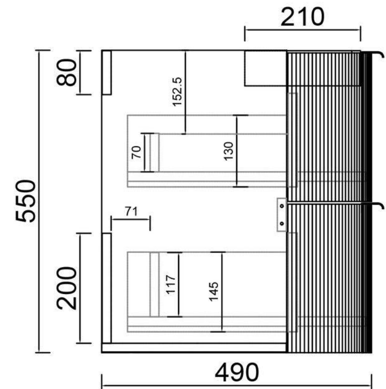
Side View
