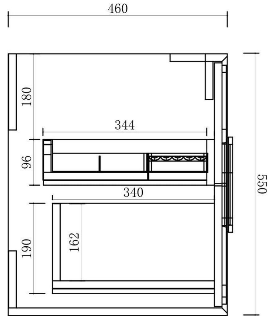
Side View
