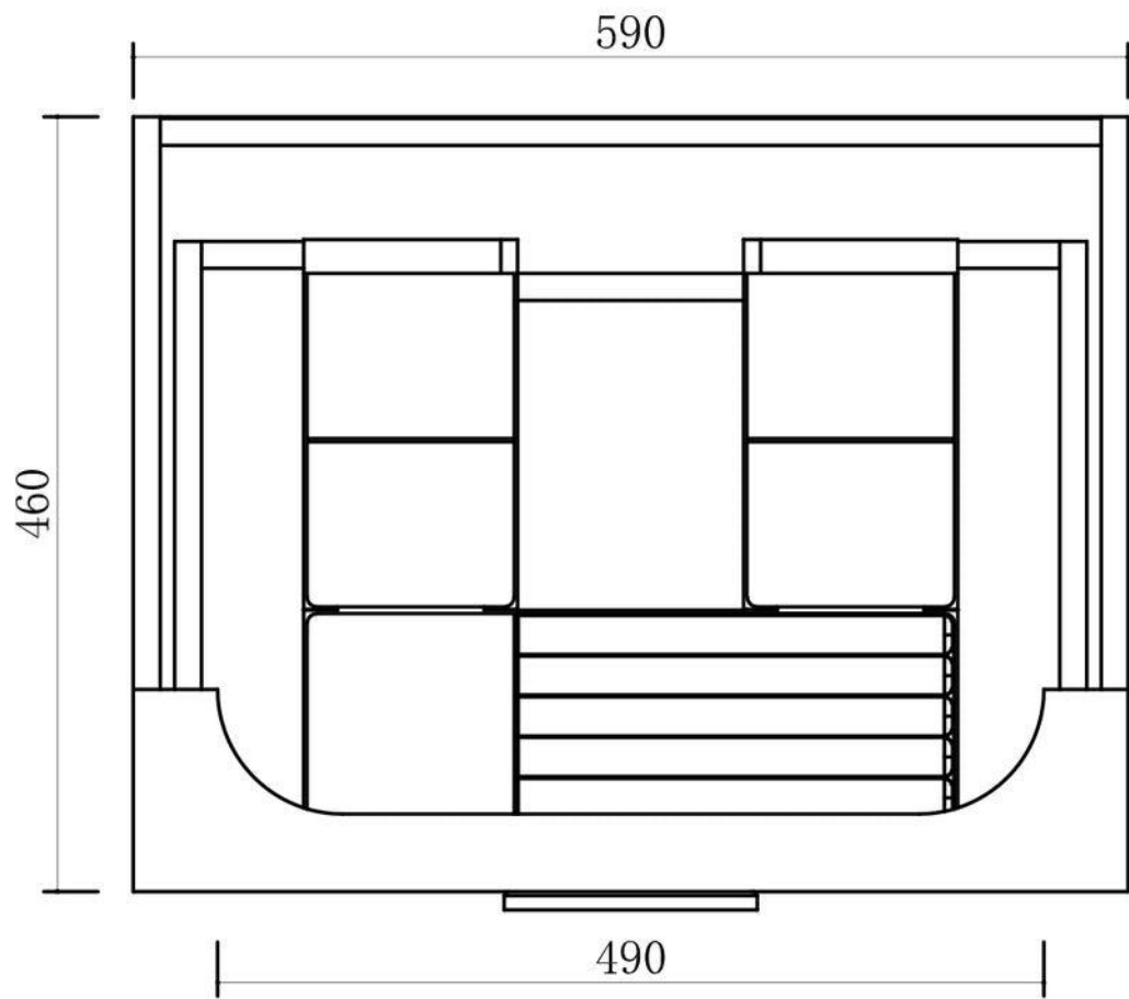
Top View
