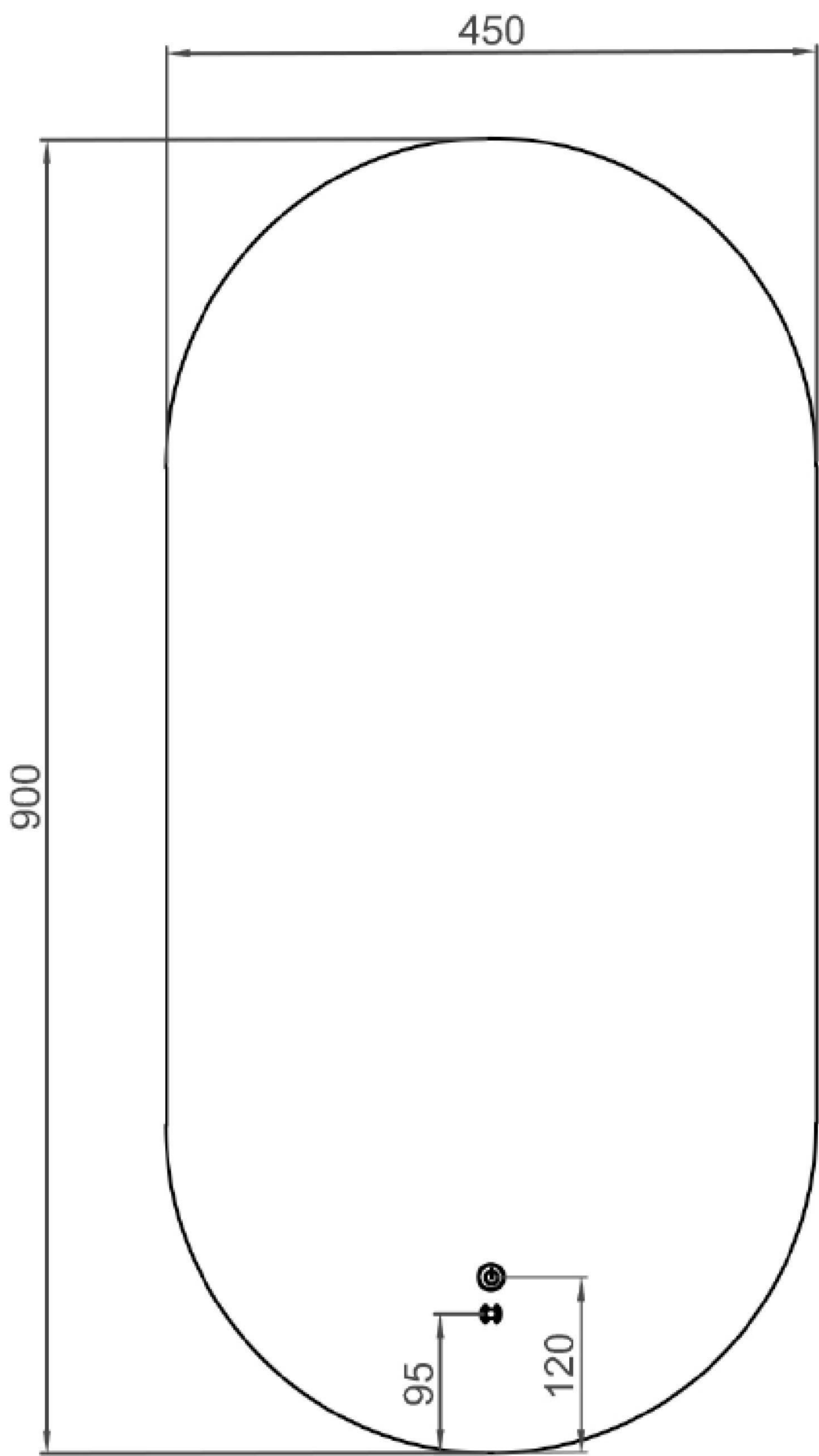
Front View
