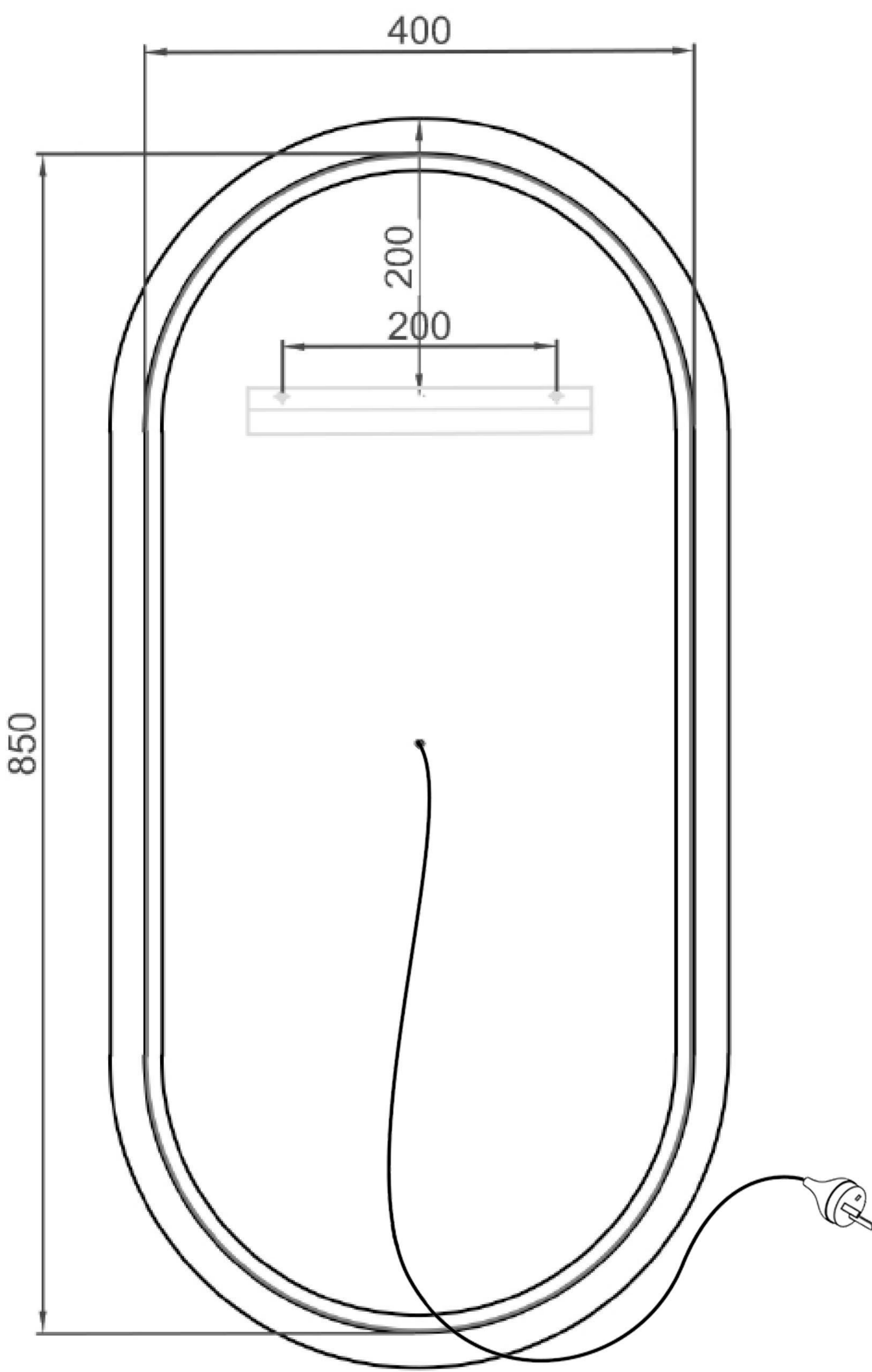
Back View
